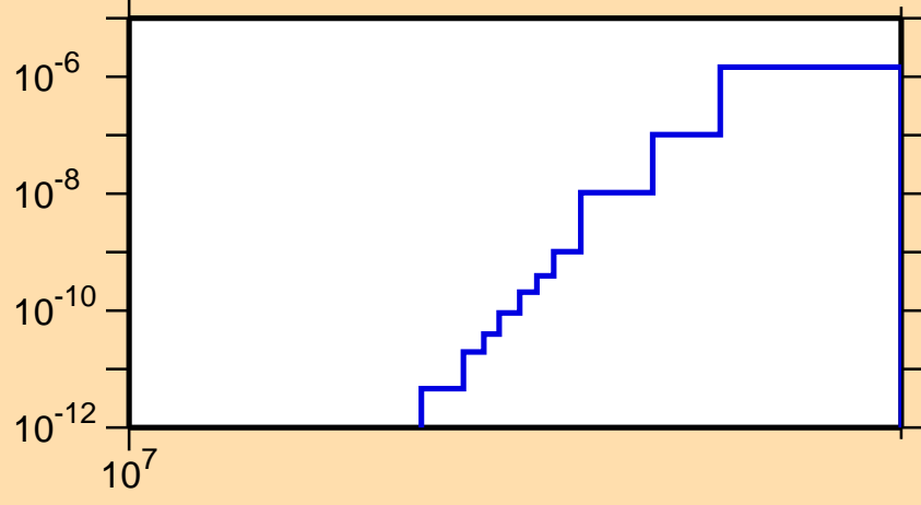
\sigma vs. E for ^{138}\text{Sm} (mt 45)
