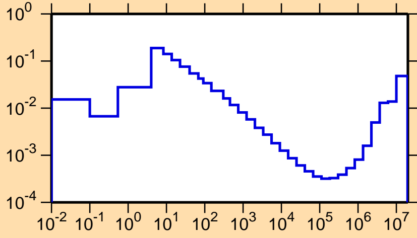
\sigma vs. E for ^{138}\text{Sm}(n,\alpha)
