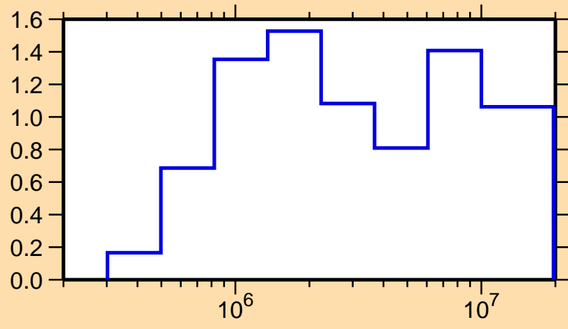
\sigma vs. E for ^{138}\text{Sm}(n,\text{inel.})
