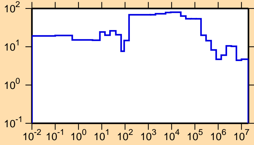
\Delta\sigma/\sigma vs. E for ^{138}\text{Sm}(n,el.)
