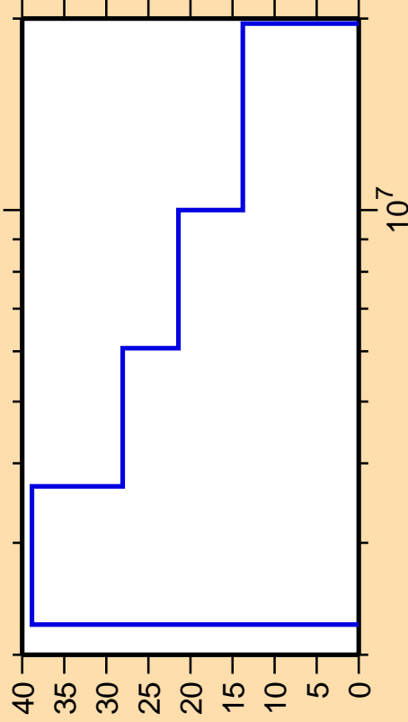
\Delta\sigma/\sigma vs. E for ^{138}\text{Sm}(n,n\text{cont.})
