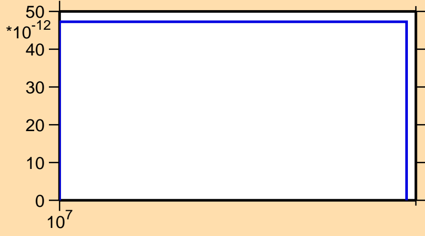
\sigma vs. E for ^{138}\text{Sm}(n,pt)
