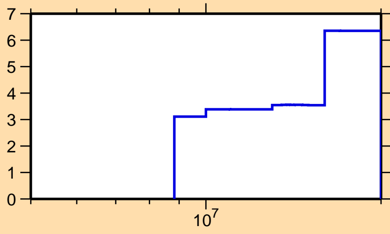
\Delta\sigma/\sigma vs. E for ^{139}\text{Sm}(n,\text{el.})
