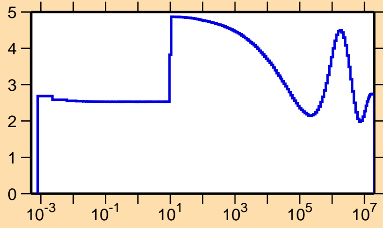
\sigma vs. E for ^{139}\text{Sm}(n,\text{el.})
