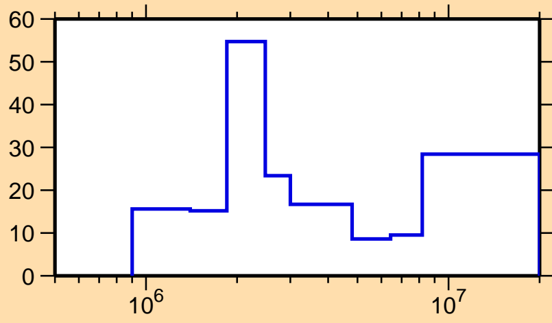
\Delta\sigma/\sigma vs. E for ^{139}\text{Sm}(n,n\text{cont.})
