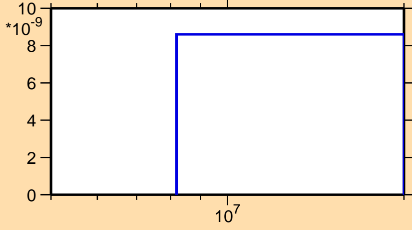
\sigma vs. E for ^{139}\text{Sm}(n,\text{pt})
