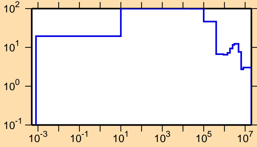
\Delta\sigma/\sigma vs. E for ^{139}\text{Sm}(n,el.)
