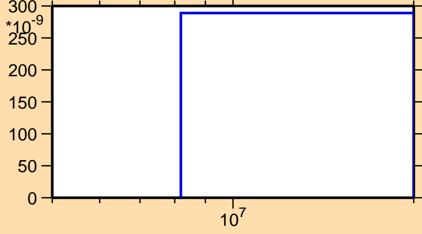
\sigma vs. E for ^{139}\text{Sm}(n,pd)
