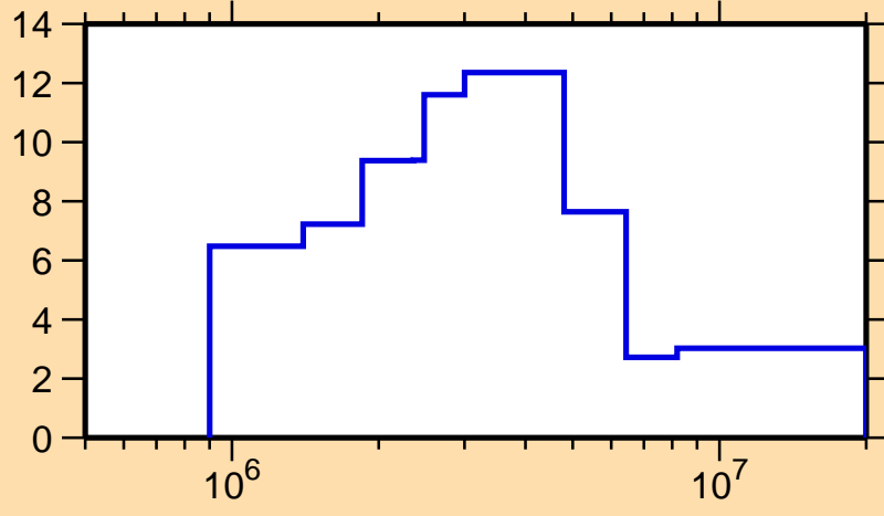
\Delta\sigma/\sigma vs. E for ^{139}\text{Sm}(n, el.)
