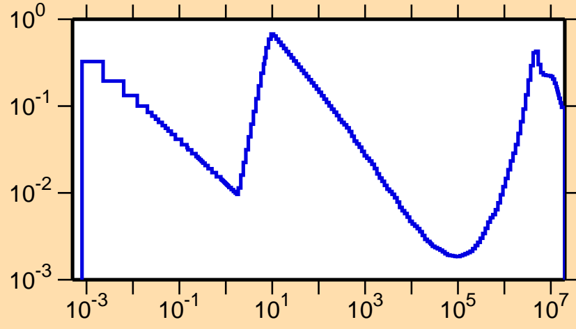
\sigma vs. E for ^{140}\text{Sm}(n,p)
