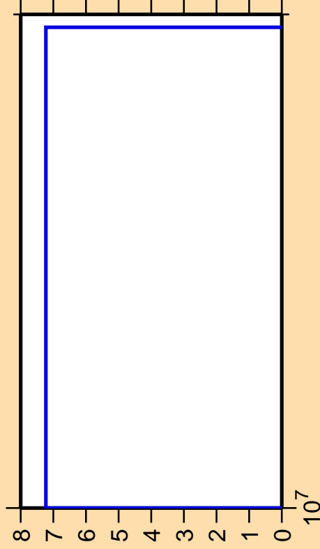
\Delta\sigma/\sigma vs. E for ^{140}\text{Sm}(n,\text{pt})
