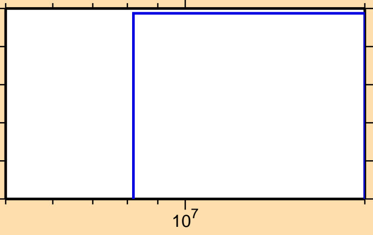
\sigma vs. E for ^{140}\text{Sm}(\text{mt } 45)
