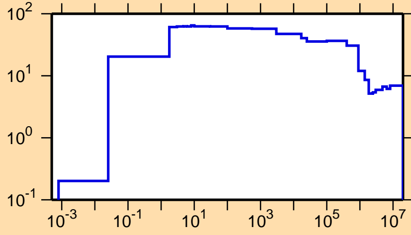
\Delta\sigma/\sigma vs. E for ^{140}\text{Sm}(n,\text{nonel.})
