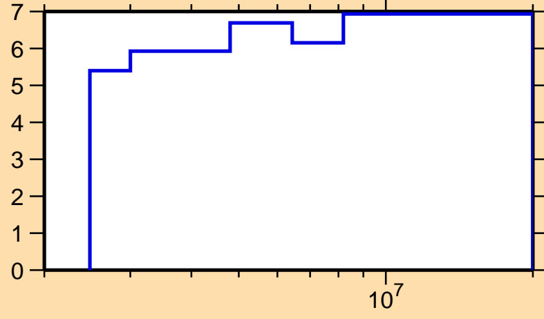
\Delta\sigma/\sigma vs. E for ^{140}\text{Sm}(n,\text{nonel.})
