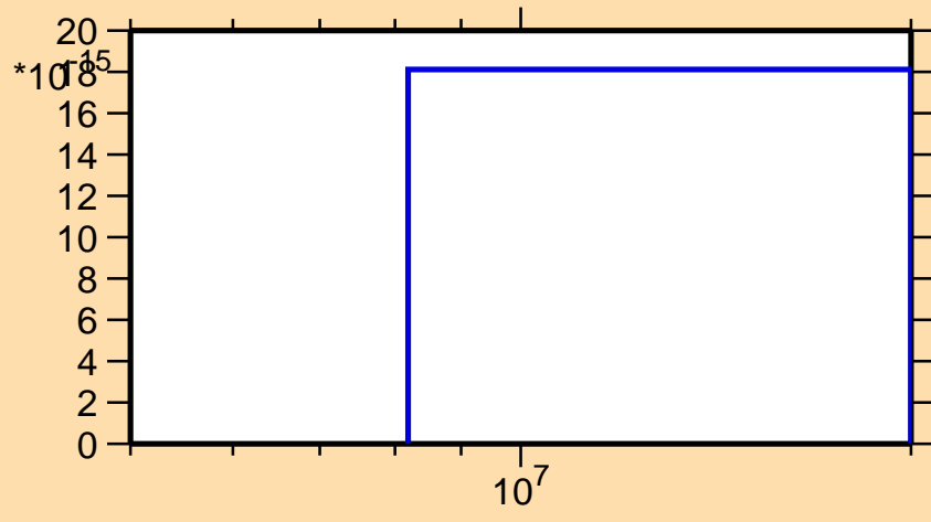
\sigma vs. E for ^{140}\text{Sm} (mt 34)
