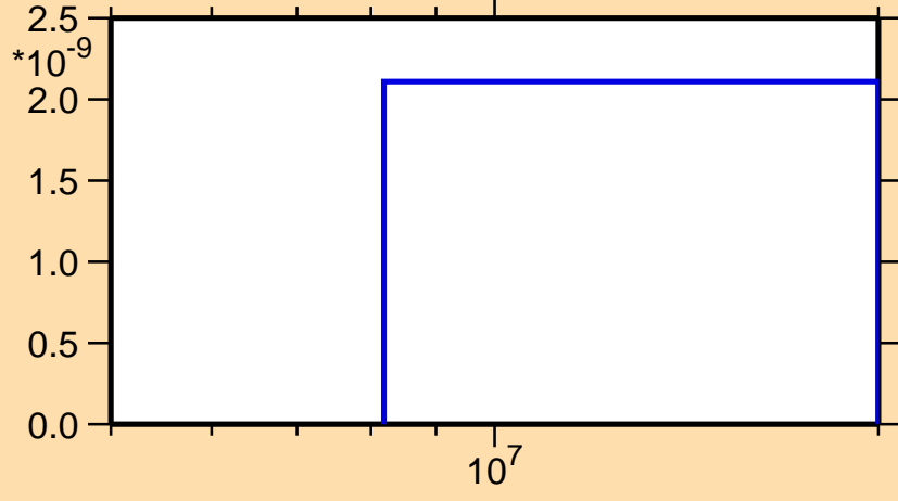
\sigma vs. E for ^{140}\text{Sm}(n,2np)
