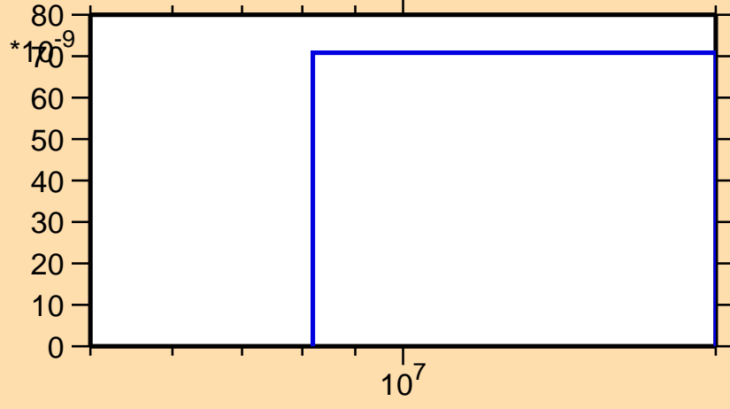
\sigma vs. E for ^{140}\text{Sm}(n,\text{pd})
