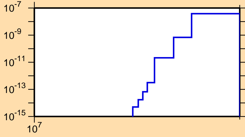
\sigma vs. E for ^{141}\text{Sm}(n,pt)
