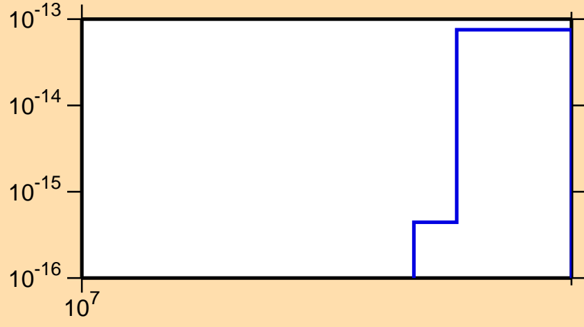
\sigma vs. E for ^{141}\text{Sm}(n,nt)
