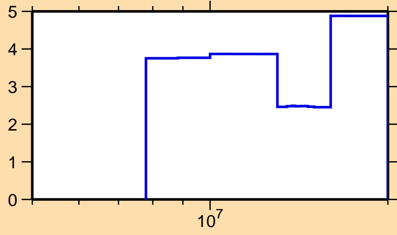
\Delta\sigma/\sigma vs. E for ^{141}\text{Sm}(n,\text{el.})
