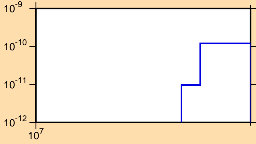
\sigma vs. E for ^{141}\text{Sm}(\text{mt117})
