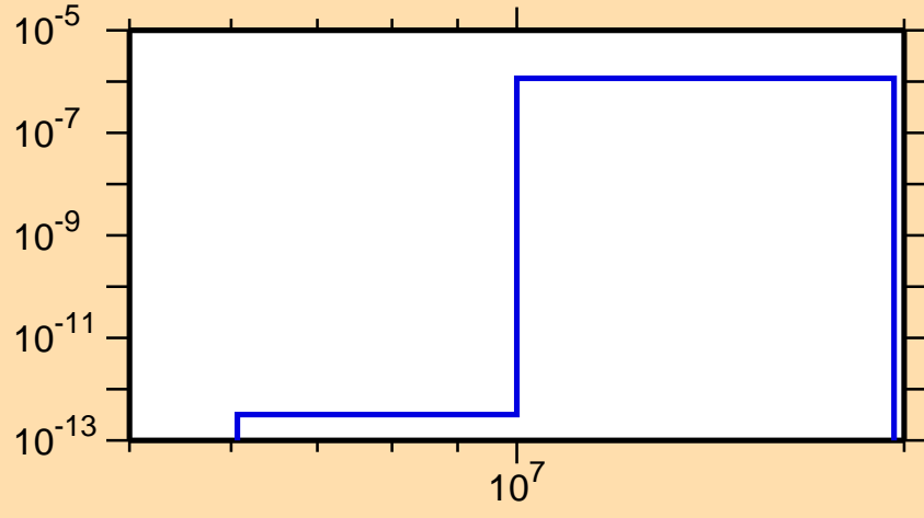
\sigma vs. E for ^{141}\text{Sm}(n,\text{He}3)
