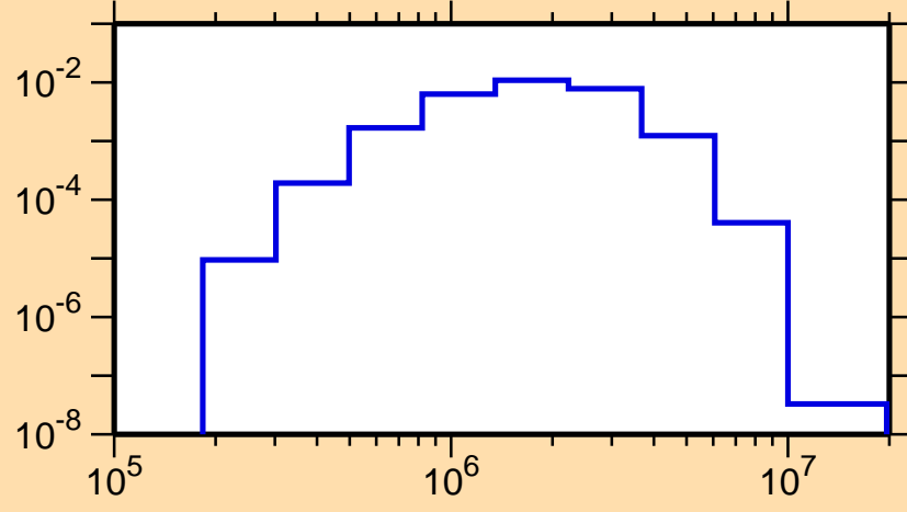
\sigma vs. E for ^{141}\text{Sm}(n,n_2)
