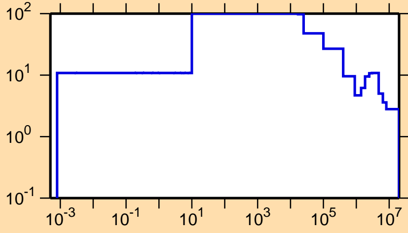
\Delta\sigma/\sigma vs. E for ^{141}\text{Sm}(n,e.l.)
