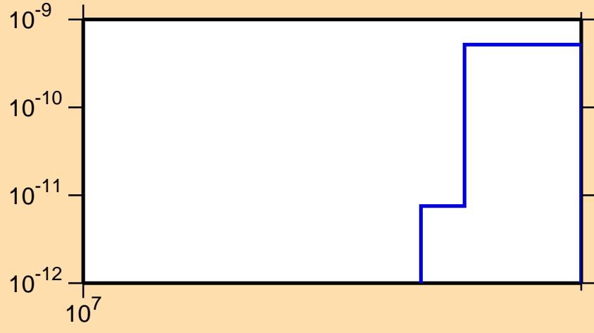
\sigma vs. E for ^{142}\text{Sm} (mt 45)
