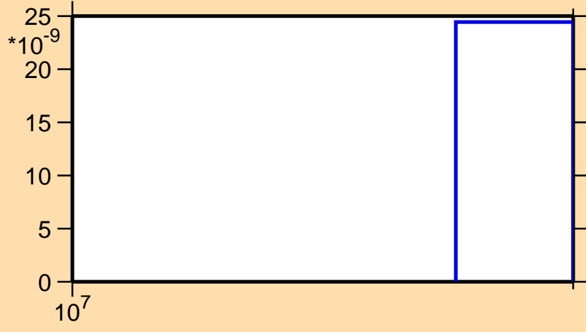
\sigma vs. E for ^{142}\text{Sm}(n,3n)
