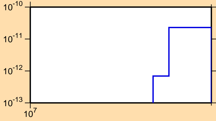
\sigma vs. E for ^{142}\text{Sm}(\text{mt117})
