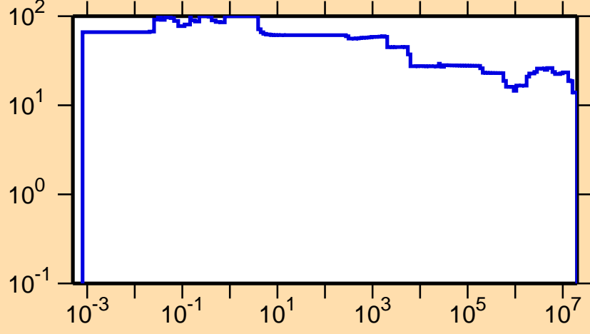
\Delta\sigma/\sigma vs. E for ^{142}\text{Sm}(n,p)
