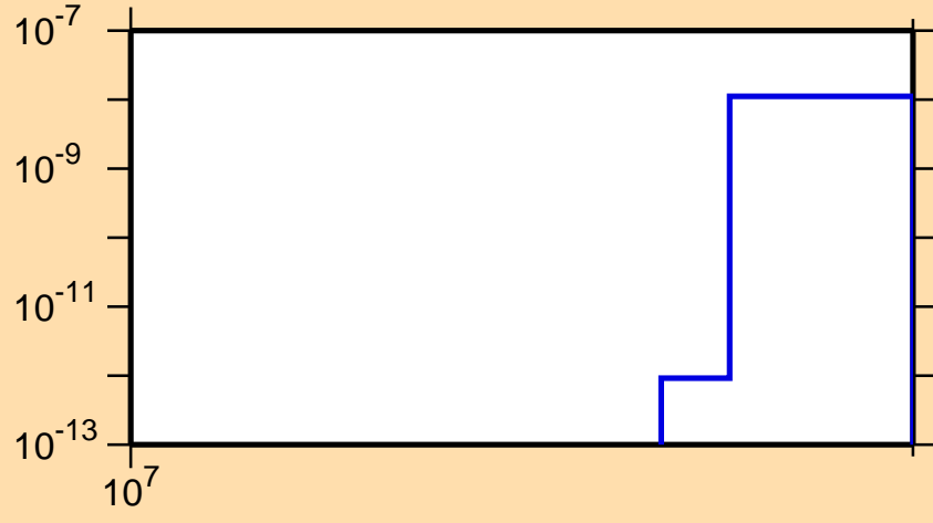
\sigma vs. E for ^{142}\text{Sm}(n,\text{nd})
