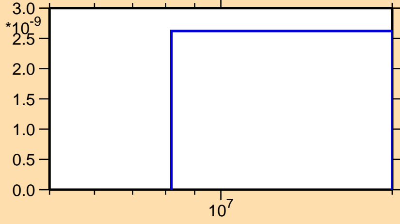
\sigma vs. E for ^{142}\text{Sm}(n,pd)
