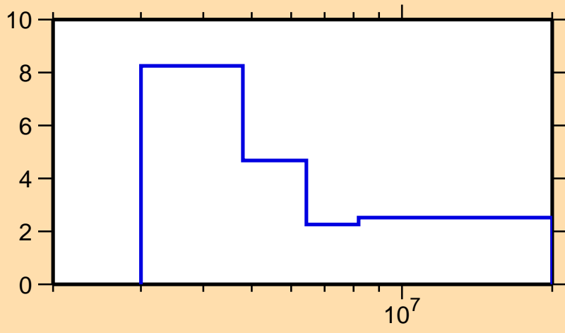
\Delta\sigma/\sigma vs. E for ^{142}\text{Sm}(n, el.)
