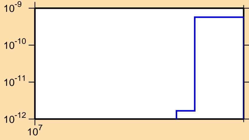
\sigma vs. E for ^{143}\text{Sm}(n,\text{pt})
