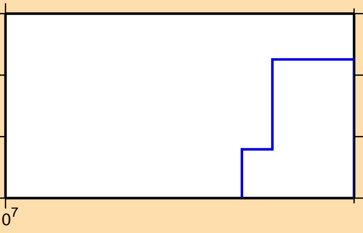
\sigma vs. E for ^{143}\text{Sm}(\text{mt117})
