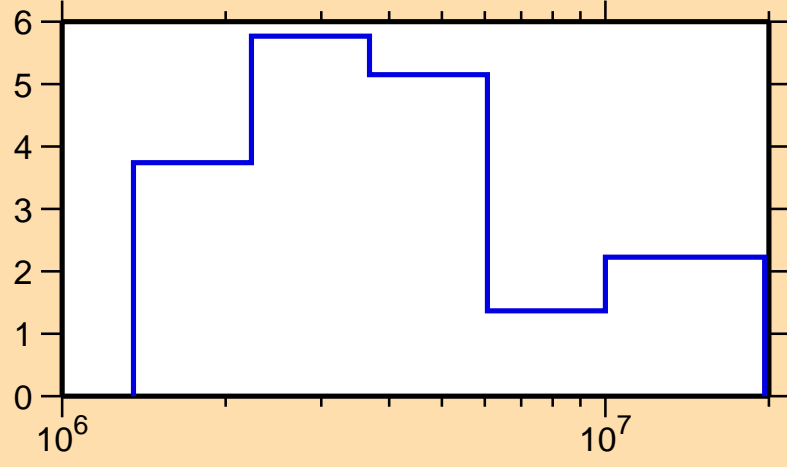
\Delta\sigma/\sigma vs. E for ^{143}\text{Sm}(n, el.)
