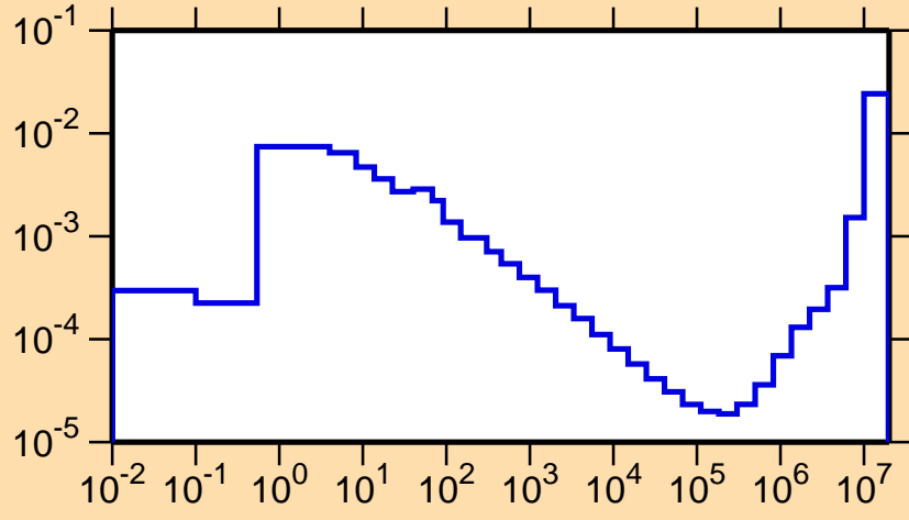
\sigma vs. E for ^{143}\text{Sm}(n,\alpha)
