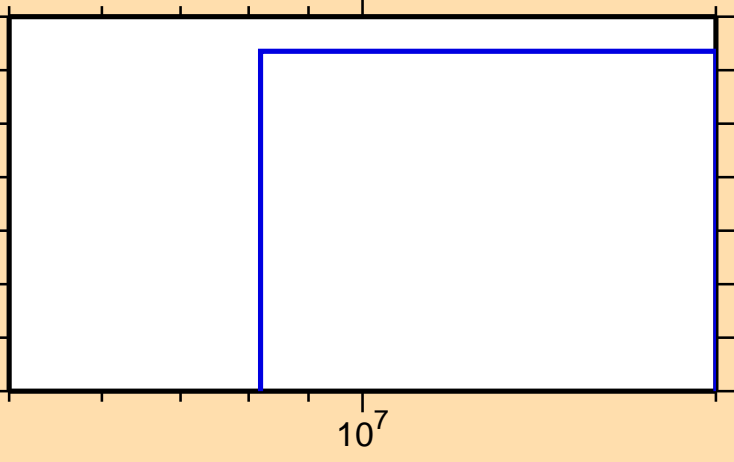
\sigma vs. E for ^{143}\text{Sm}(n,2n\alpha)
