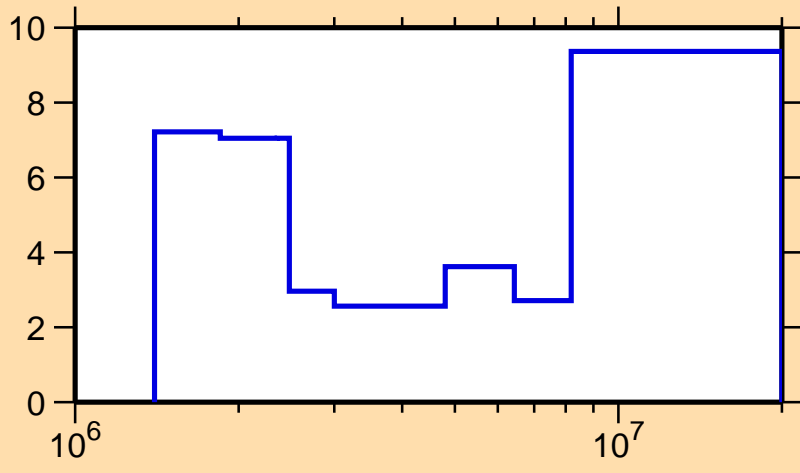
\Delta\sigma/\sigma vs. E for ^{143}\text{Sm}(n,ncont.)
