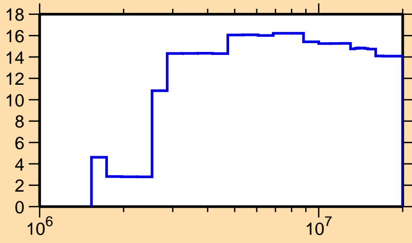
\Delta\sigma/\sigma vs. E for ^{144}\text{Sm}(n,n_1)
