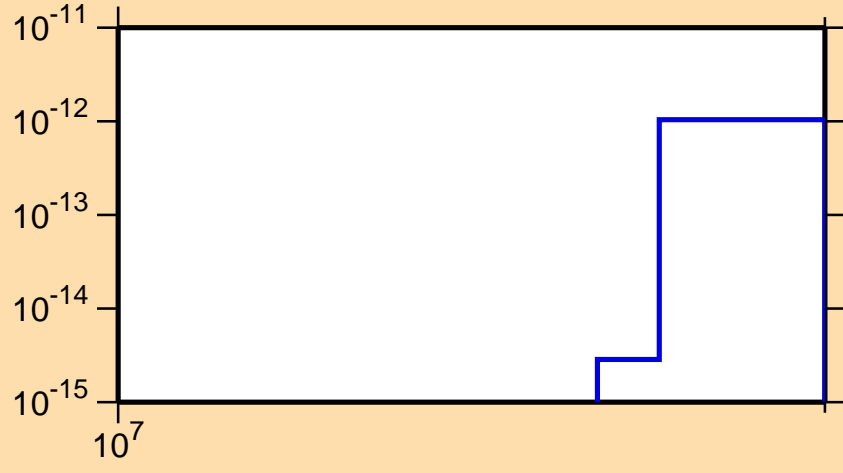
\sigma vs. E for ^{144}\text{Sm} (mt 45)
