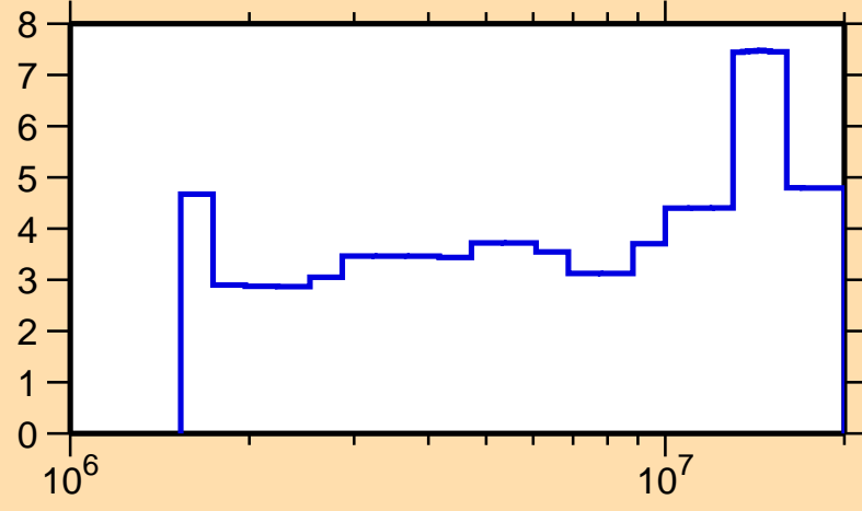
\Delta\sigma/\sigma vs. E for ^{144}\text{Sm}(n,\text{inel.})
