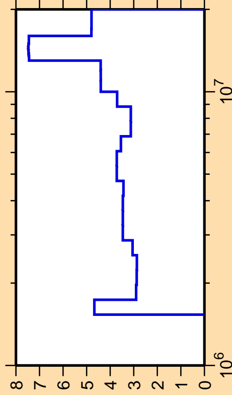
\Delta\sigma/\sigma vs. E for ^{144}\text{Sm}(n,\text{inel.})
