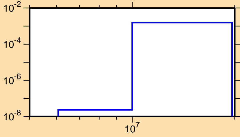
\sigma vs. E for ^{144}\text{Sm}(n,d)
