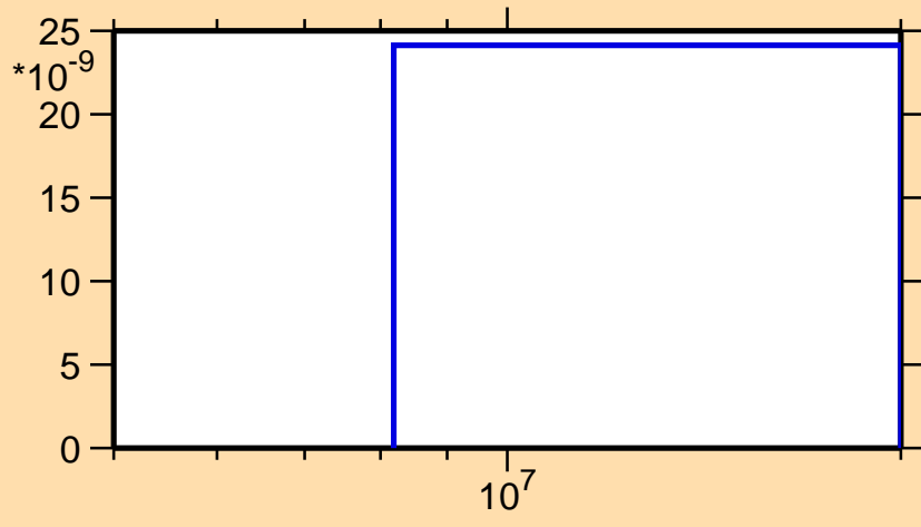
\sigma vs. E for ^{144}\text{Sm}(n,p\alpha)
