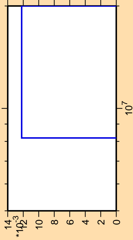
\Delta\sigma/\sigma vs. E for ^{144}\text{Sm}(\text{mt117})
