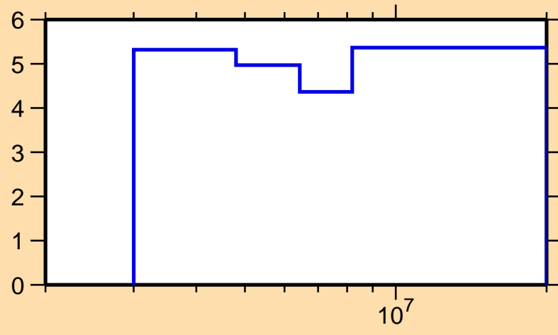
\Delta\sigma/\sigma vs. E for ^{144}\text{Sm}(n,n\text{cont.})
