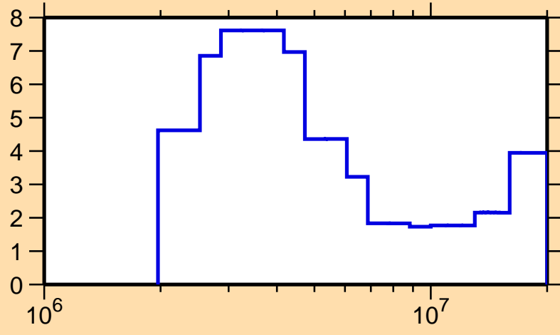
\Delta\sigma/\sigma vs. E for ^{145}\text{Sm}(n, el.)
