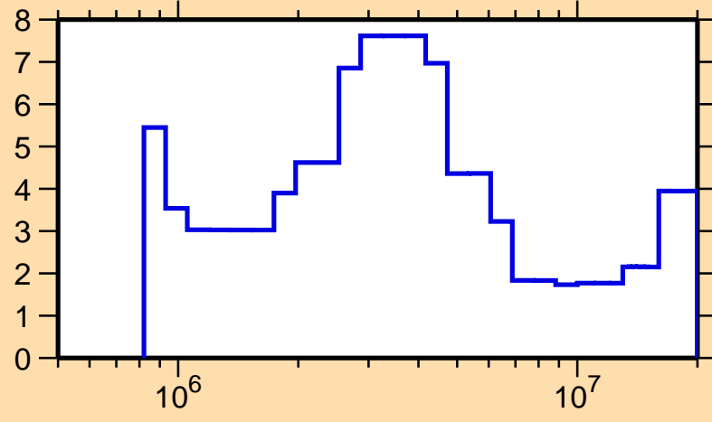
\Delta\sigma/\sigma vs. E for ^{145}\text{Sm}(n,\text{el.})
