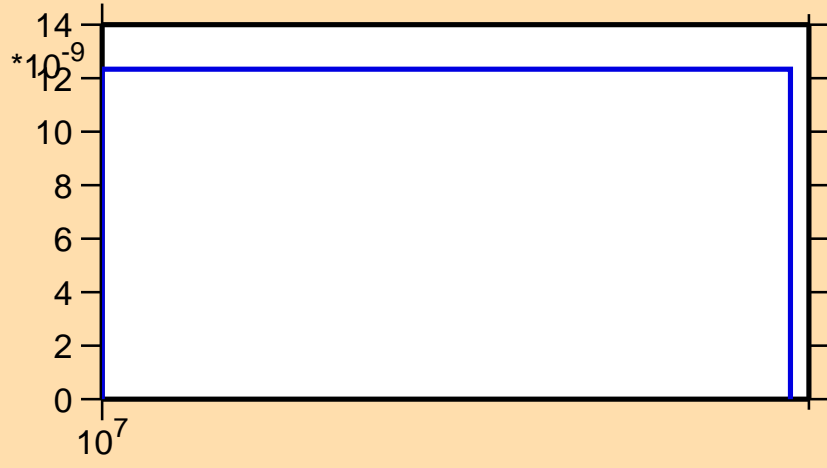
\sigma vs. E for ^{145}\text{Sm}(n,2n\alpha)
