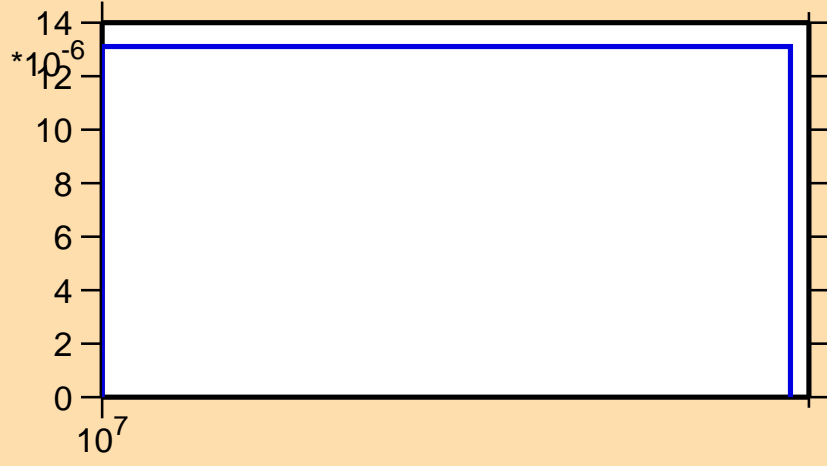
\sigma vs. E for ^{145}\text{Sm}(n,3n)
