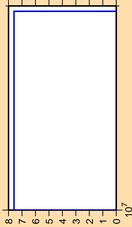
\Delta\sigma/\sigma vs. E for ^{145}\text{Sm}(n,nt)
