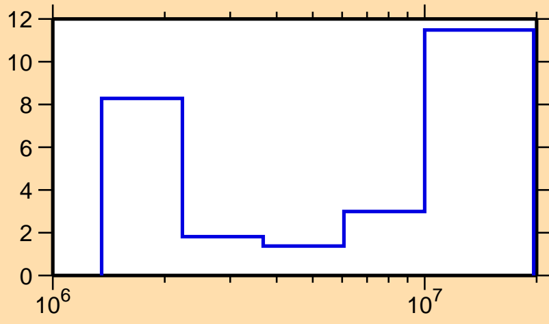
\Delta\sigma/\sigma vs. E for ^{145}\text{Sm}(n,incl.)
