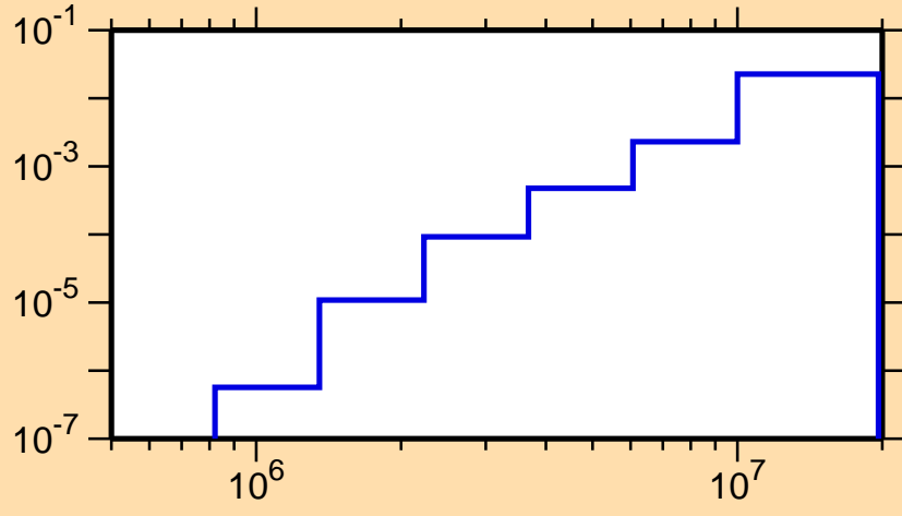
\sigma vs. E for ^{145}\text{Sm}(n,p)
