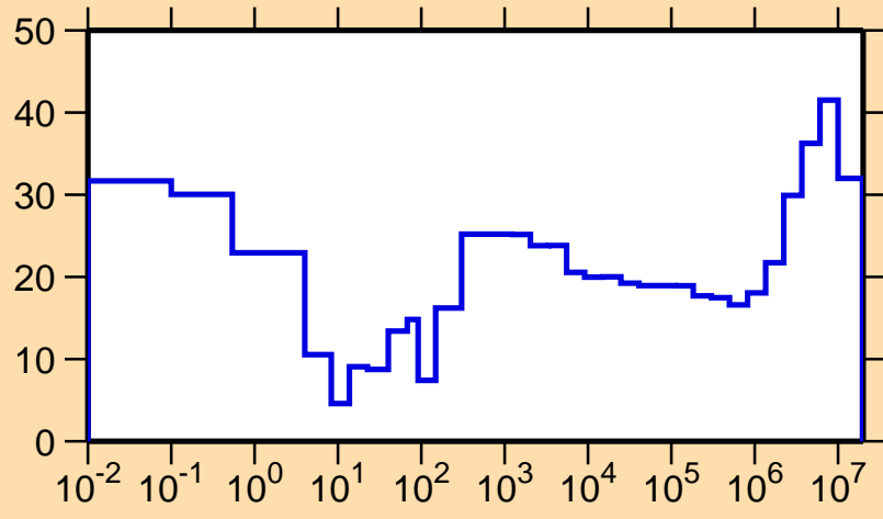
\Delta\sigma/\sigma vs. E for ^{145}\text{Sm}(n,\gamma)
