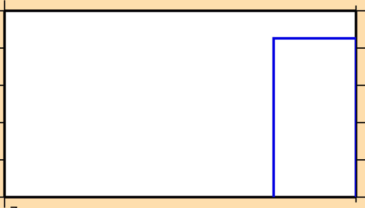
\sigma vs. E for ^{146}\text{Sm} (mt 11)
