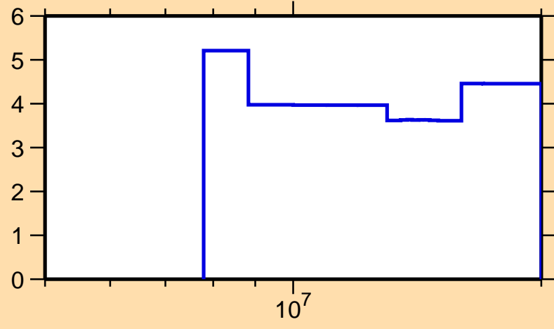
\Delta\sigma/\sigma vs. E for ^{146}\text{Sm}(n,2n)
