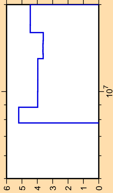
\Delta\sigma/\sigma vs. E for ^{146}\text{Sm}(n,2n)
