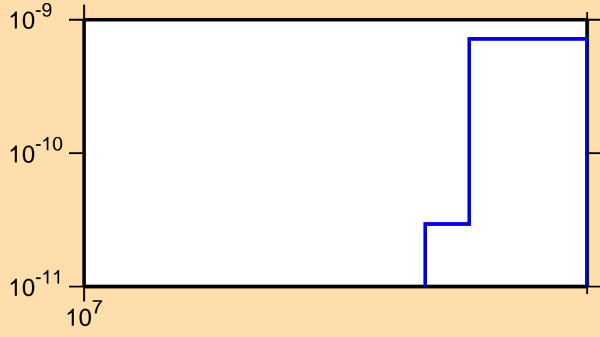
\sigma vs. E for ^{146}\text{Sm} (mt 45)
