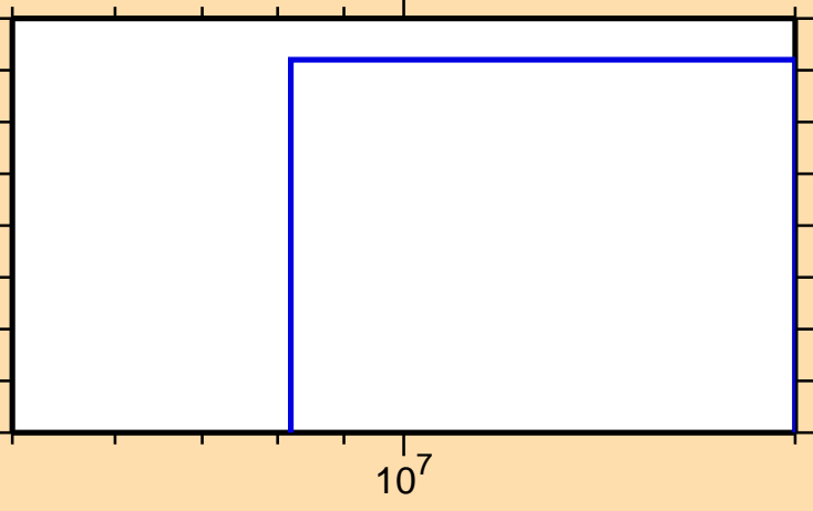
\sigma vs. E for ^{146}\text{Sm} (mt 45)
