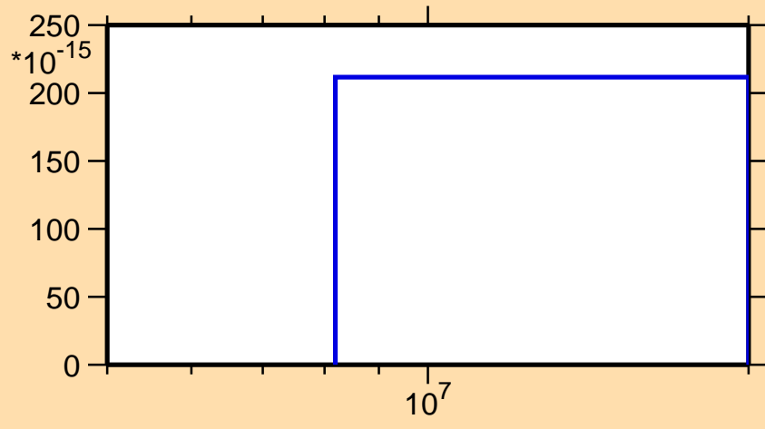
\sigma vs. E for ^{146}\text{Sm}(n,pd)
