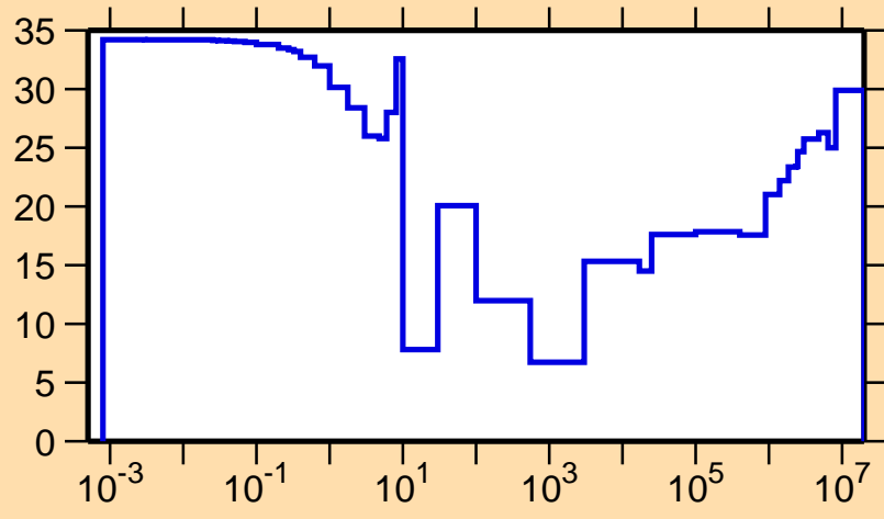
\Delta\sigma/\sigma vs. E for ^{146}\text{Sm}(n,\gamma)
