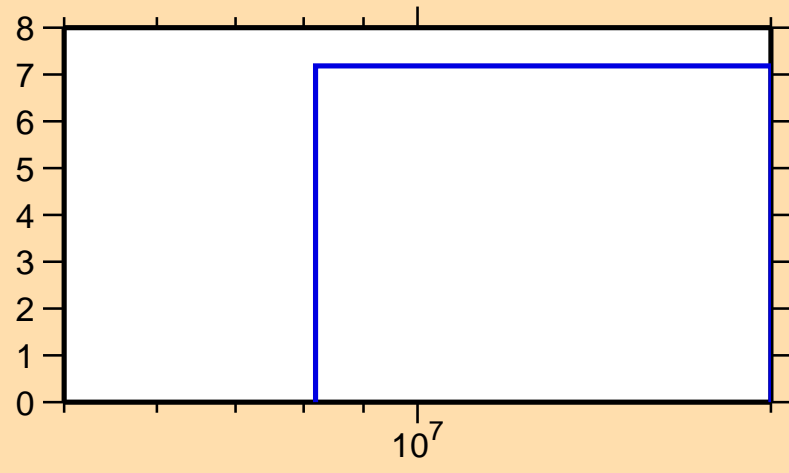
\Delta\sigma/\sigma vs. E for ^{146}\text{Sm}(n,\text{inel.})
