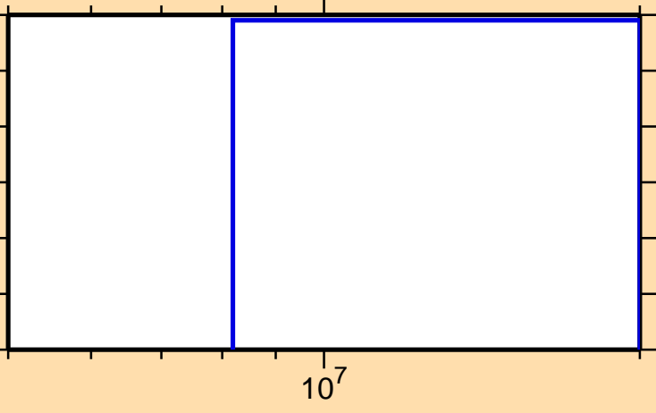
\sigma vs. E for ^{146}\text{Sm}(n,t)
