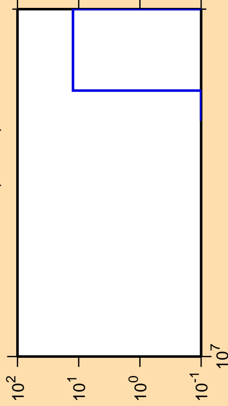
\Delta\sigma/\sigma vs. E for ^{147}\text{Sm} (mt 34)
