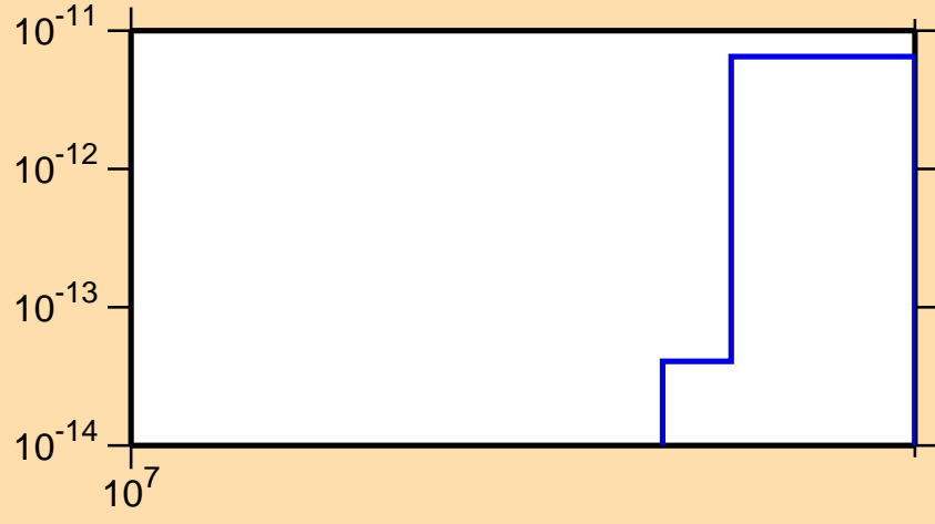
\sigma vs. E for ^{147}\text{Sm}(n,pt)
