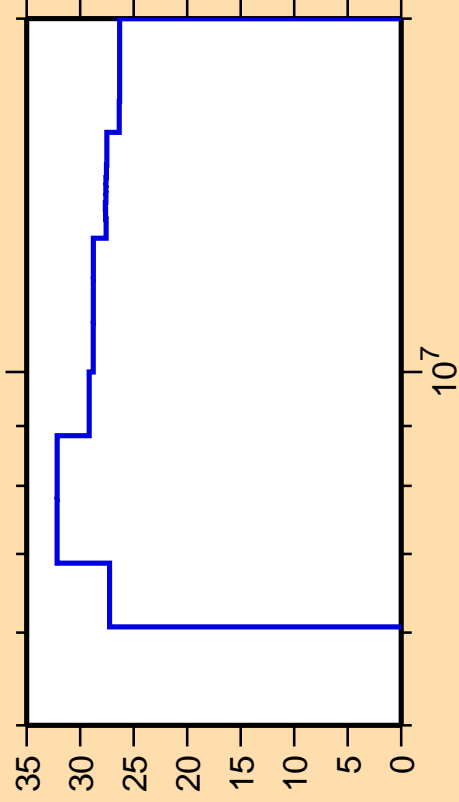
\Delta\sigma/\sigma vs. E for ^{147}\text{Sm}(n,p)
