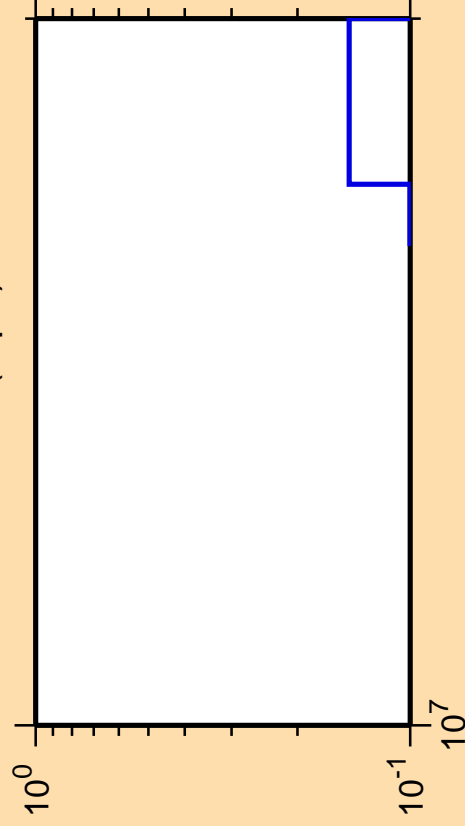
\Delta\sigma/\sigma vs. E for ^{147}\text{Sm}(n,pd)
