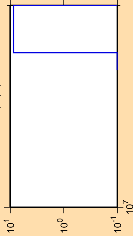
\Delta\sigma/\sigma vs. E for ^{147}\text{Sm}(n,pt)
