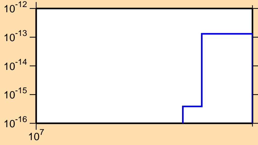
\sigma vs. E for ^{147}\text{Sm}(n,pd)
