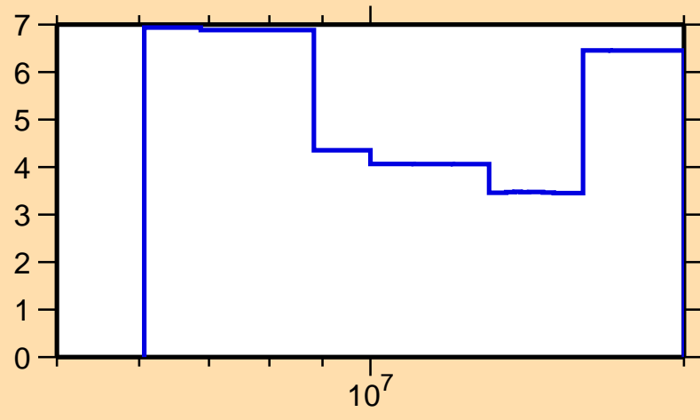
\Delta\sigma/\sigma vs. E for ^{147}\text{Sm}(n,2n)
