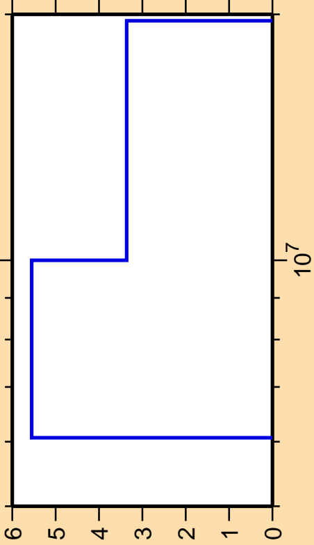
\Delta\sigma/\sigma vs. E for ^{147}\text{Sm}(n,2n)
