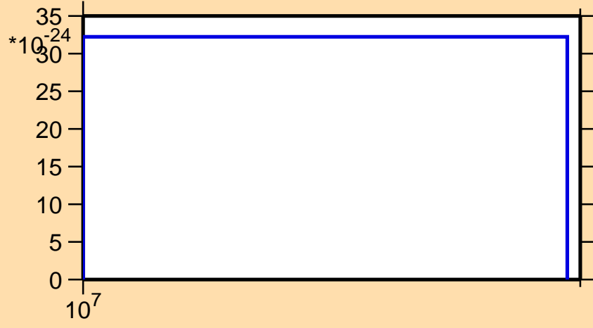
\sigma vs. E for ^{147}\text{Sm} (mt 11)
