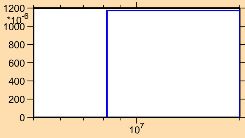
\sigma vs. E for ^{147}\text{Sm}(n,np)
