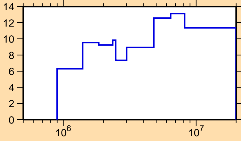
\Delta\sigma/\sigma vs. E for ^{147}\text{Sm}(n,n_1)
