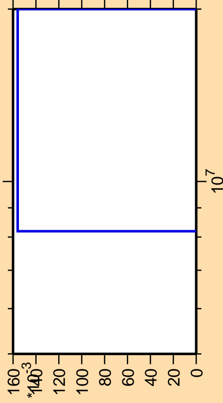
\Delta\sigma/\sigma vs. E for ^{147}\text{Sm} (mt 45)
