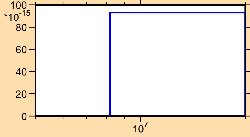
\sigma vs. E for ^{147}\text{Sm} (mt 45)
