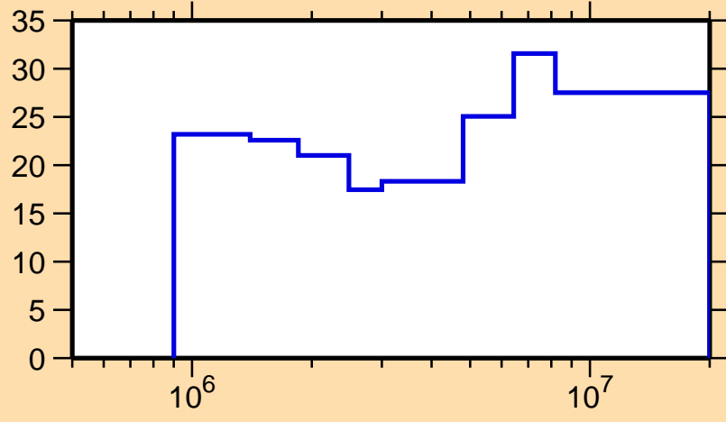
\Delta\sigma/\sigma vs. E for ^{147}\text{Sm}(n,p)
