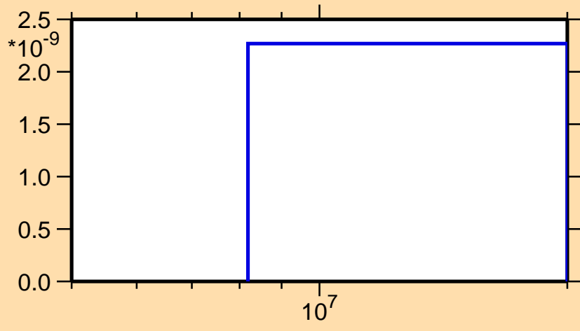
\sigma vs. E for ^{147}\text{Sm}(n,nt)
