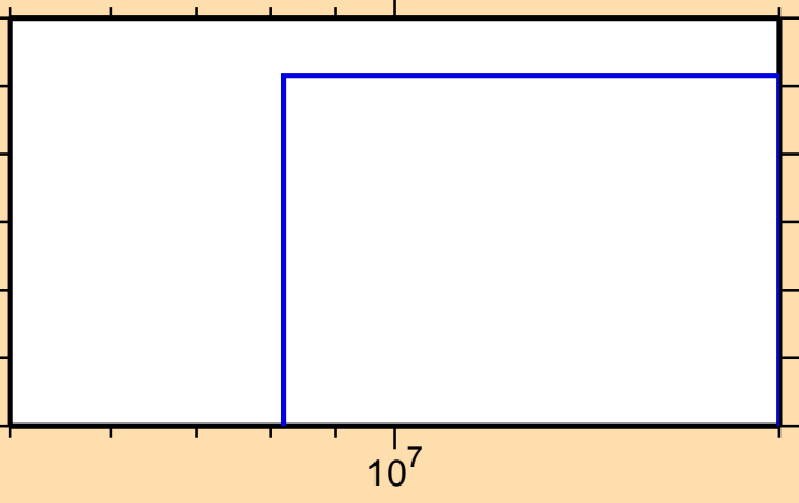
\sigma vs. E for ^{147}\text{Sm}(n,\text{He}3)
