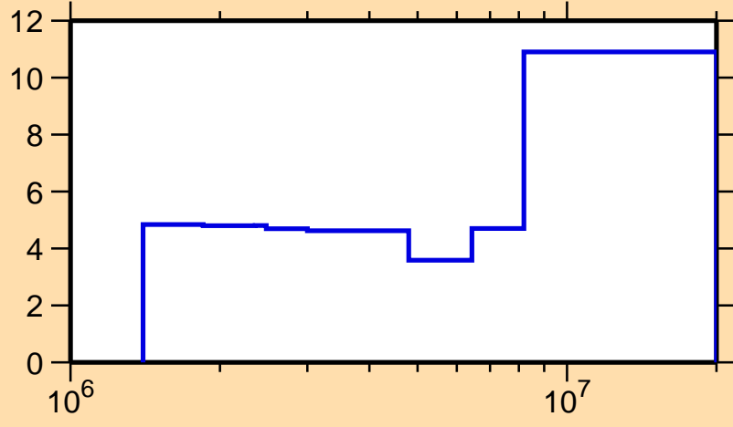
\Delta\sigma/\sigma vs. E for ^{147}\text{Sm}(n,ncont.)
