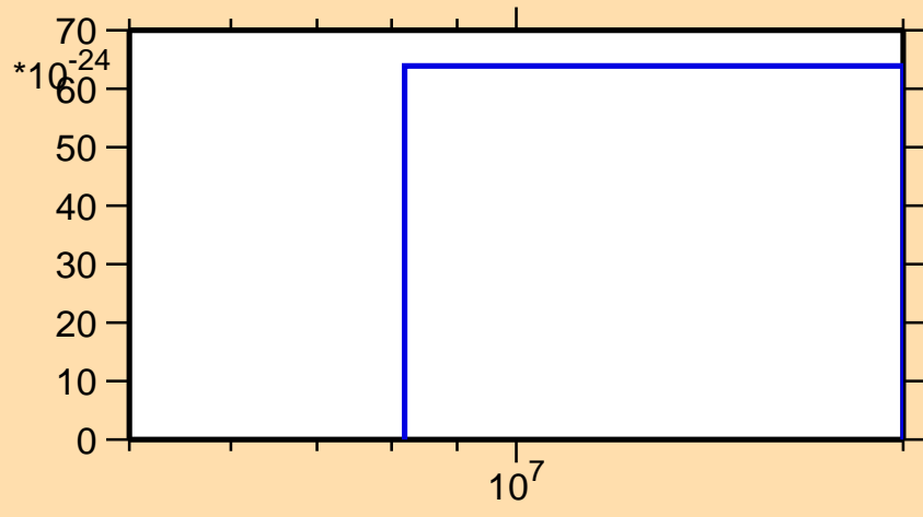
\sigma vs. E for ^{147}\text{Sm} (mt 11)
