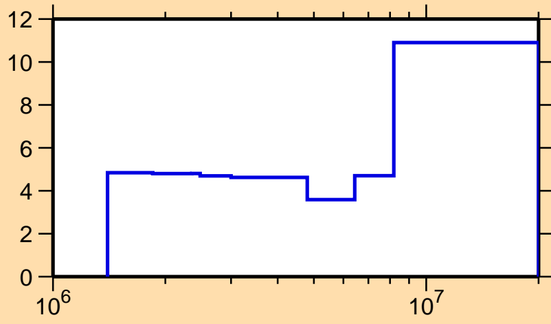
\Delta\sigma/\sigma vs. E for ^{147}\text{Sm}(n,n\text{cont.})
