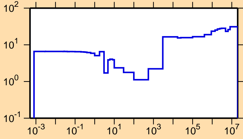
\Delta\sigma/\sigma vs. E for ^{147}\text{Sm}(n,\gamma)
