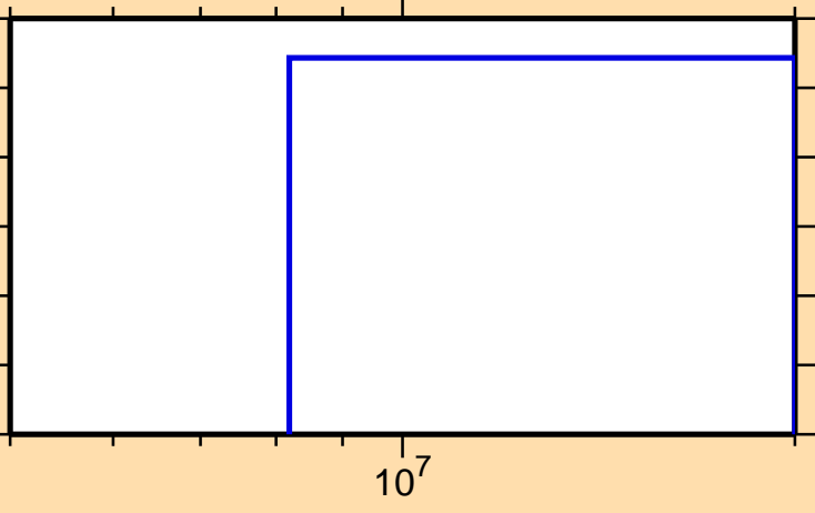
\sigma vs. E for ^{147}\text{Sm}(n,\text{pt})
