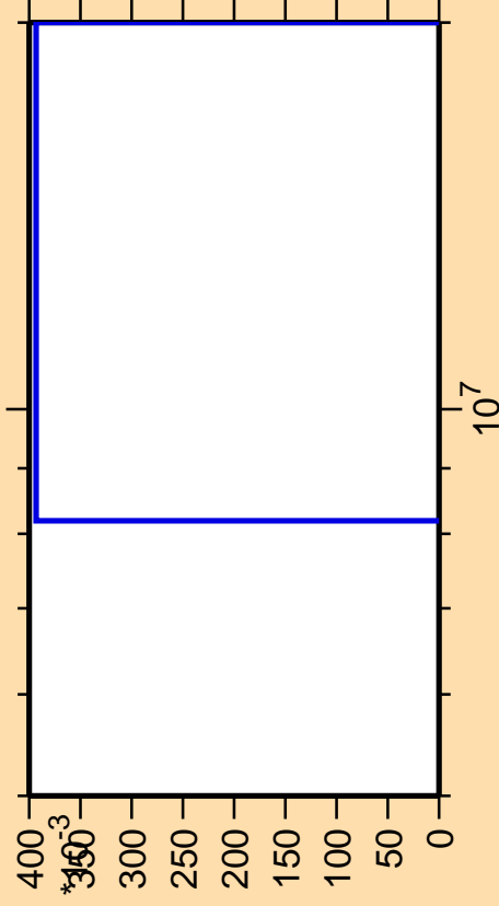
\Delta\sigma/\sigma vs. E for ^{147}\text{Sm}(\text{mt117})
