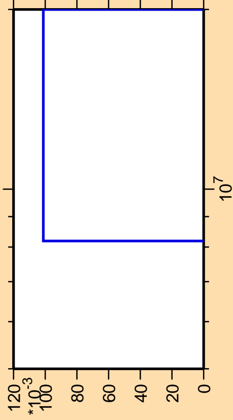
\Delta\sigma/\sigma vs. E for ^{147}\text{Sm} (mt 34)
