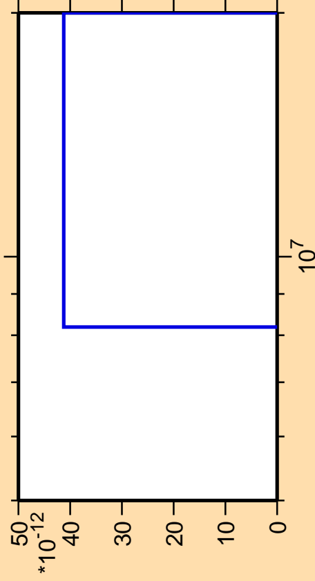
\Delta\sigma/\sigma vs. E for ^{147}\text{Sm} (mt 11)
