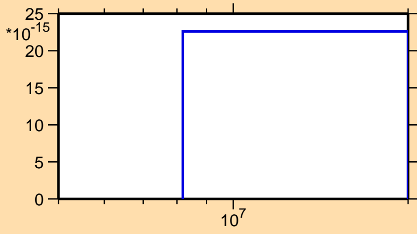
\sigma vs. E for ^{147}\text{Sm} (mt 34)
