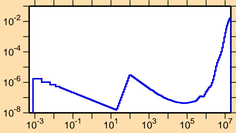
\sigma vs. E for ^{148}\text{Sm}(n,\alpha)
