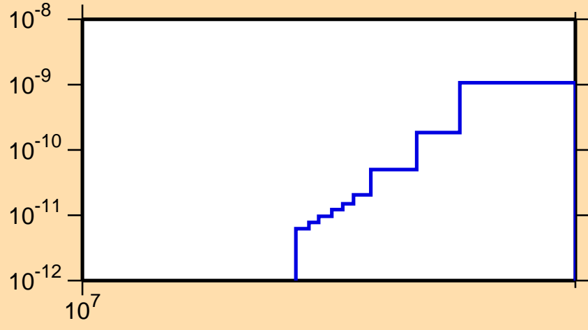
\sigma vs. E for ^{148}\text{Sm}(n,p\alpha)
