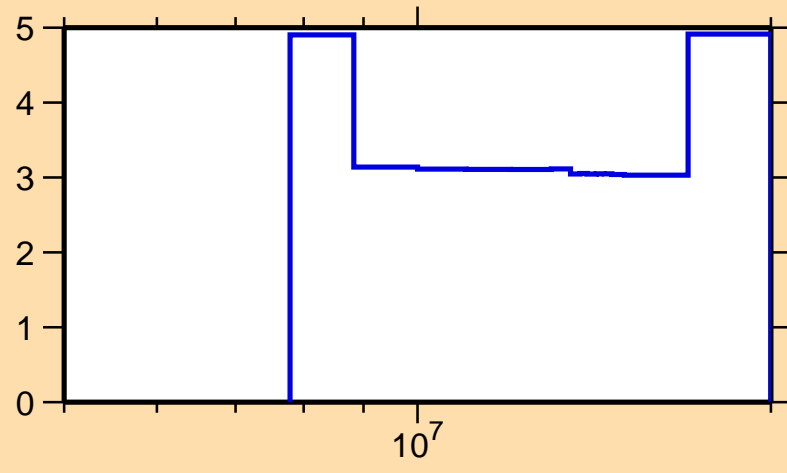
\Delta\sigma/\sigma vs. E for ^{148}\text{Sm}(n,2n)
