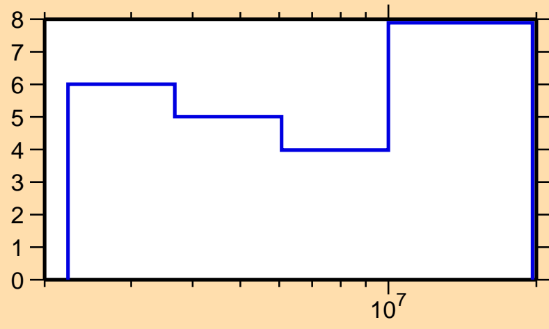
\Delta\sigma/\sigma vs. E for ^{148}\text{Sm}(n,n\text{cont.})
