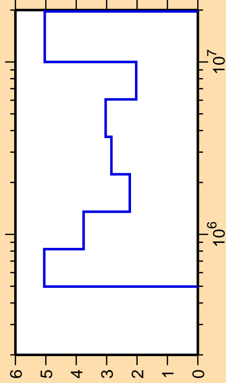
\Delta\sigma/\sigma vs. E for ^{148}\text{Sm}(n,\text{inel.})
