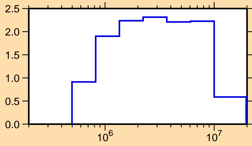
\sigma vs. E for ^{148}\text{Sm}(n,\text{inel.})
