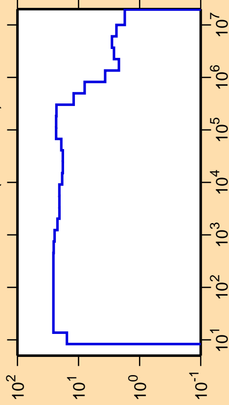
\Delta\sigma/\sigma vs. E for ^{148}\text{Sm}(n,\text{nonel.})
