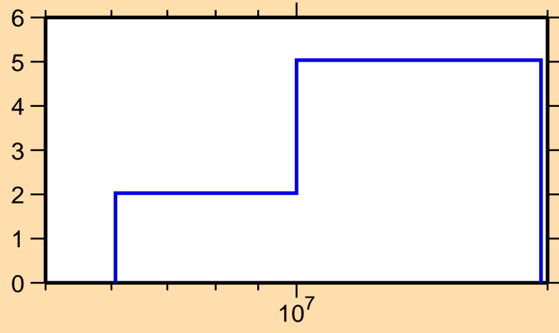
\Delta\sigma/\sigma vs. E for ^{148}\text{Sm}(n,\text{inel.})
