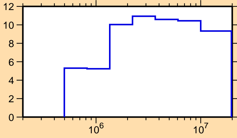
\Delta\sigma/\sigma vs. E for ^{148}\text{Sm}(n,n_1)
