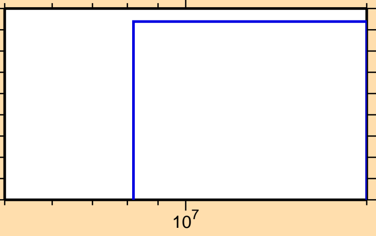
\sigma vs. E for ^{148}\text{Sm}(n,np)
