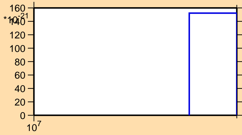
\sigma vs. E for ^{149}\text{Sm} (mt 11)
