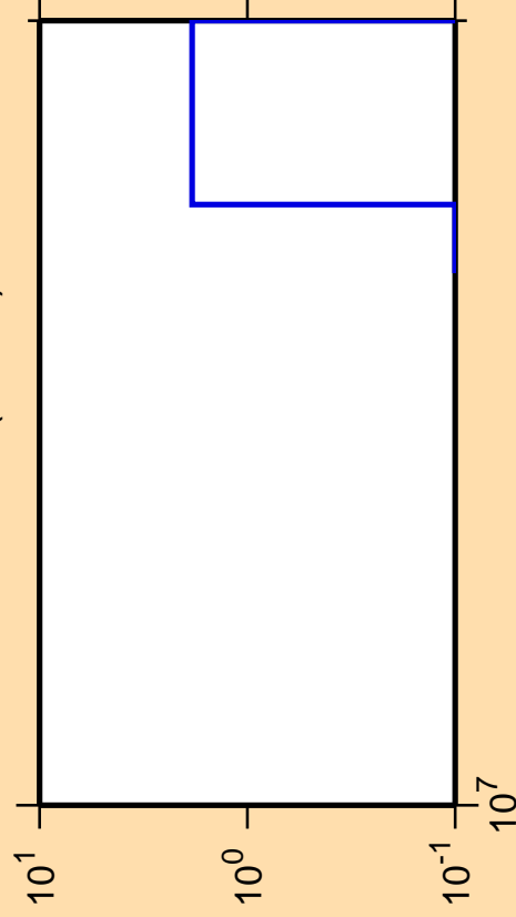
\Delta\sigma/\sigma vs. E for ^{149}\text{Sm} (mt 34)
