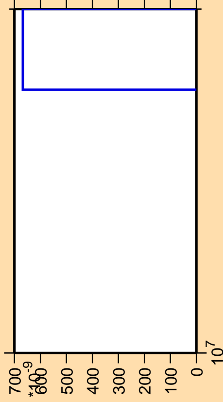
\Delta\sigma/\sigma vs. E for ^{149}\text{Sm} (mt 11)
