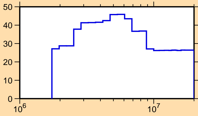
\Delta\sigma/\sigma vs. E for ^{149}\text{Sm}(n,\gamma)
