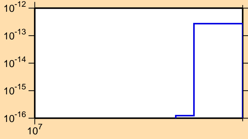
\sigma vs. E for ^{149}\text{Sm} (mt 34)
