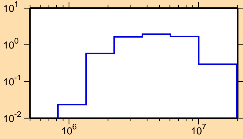
\sigma vs. E for ^{149}\text{Sm}(n,n\text{cont.})
