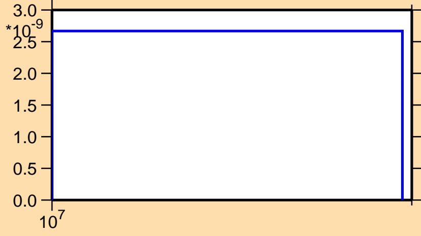
\sigma vs. E for ^{149}\text{Sm}(n,nt)
