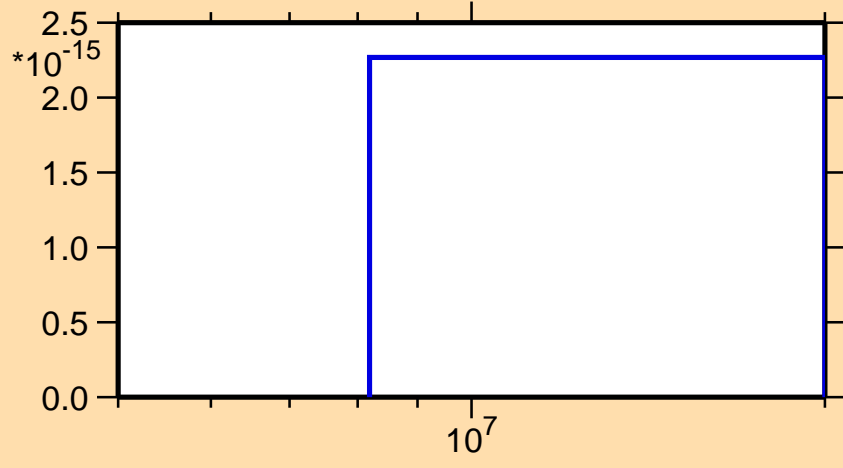
\sigma vs. E for ^{149}\text{Sm} (mt 34)
