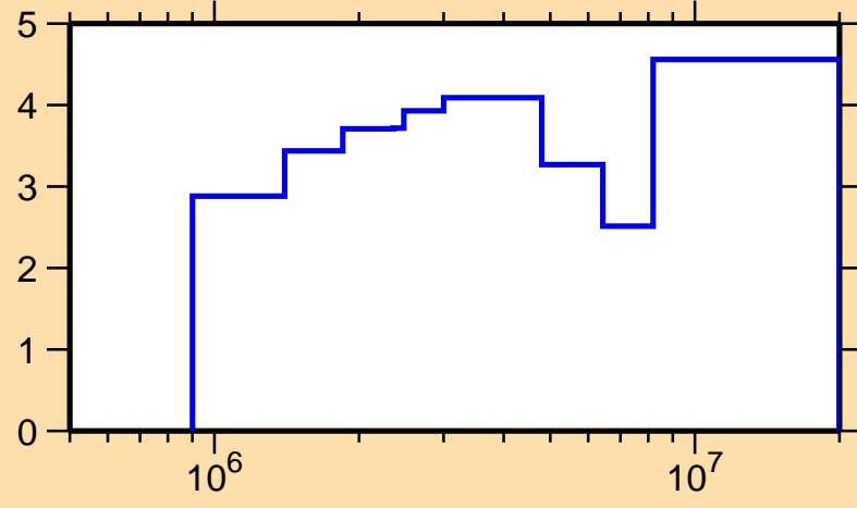
\Delta\sigma/\sigma vs. E for ^{149}\text{Sm}(n,\text{inel.})
