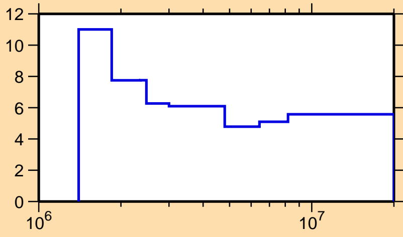
\Delta\sigma/\sigma vs. E for ^{149}\text{Sm}(n,n\text{cont.})
