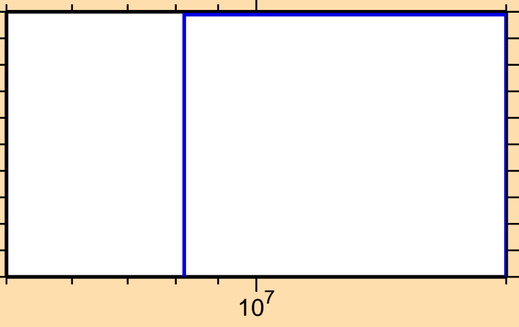
\sigma vs. E for ^{149}\text{Sm}(n,p\alpha)
