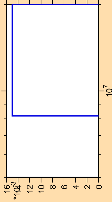
\Delta\sigma/\sigma vs. E for ^{149}\text{Sm} (mt 34)
