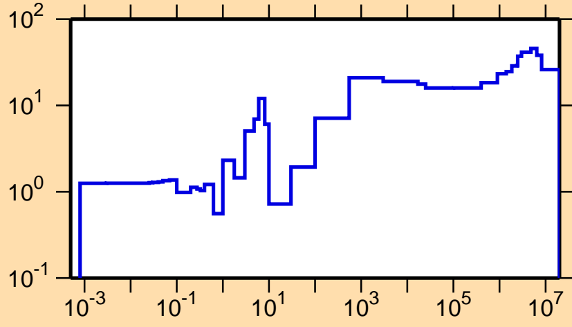
\Delta\sigma/\sigma vs. E for ^{149}\text{Sm}(n,\gamma)
