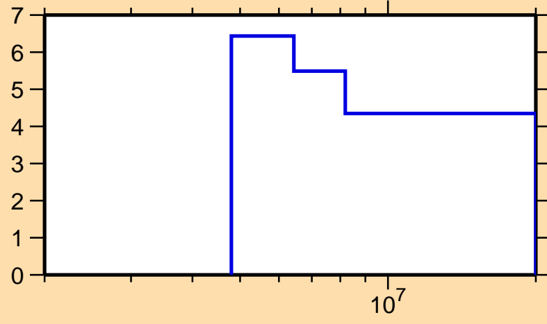
\Delta\sigma/\sigma vs. E for ^{149}\text{Sm}(n,2n)
