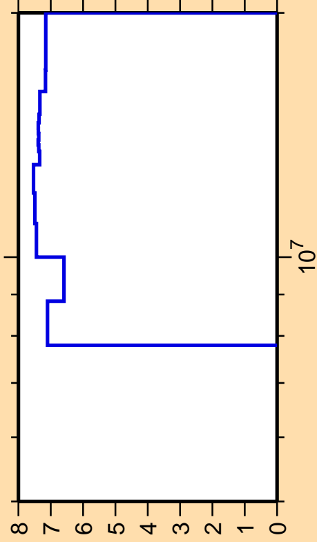
\Delta\sigma/\sigma vs. E for ^{150}\text{Sm}(n,n\text{cont.})
