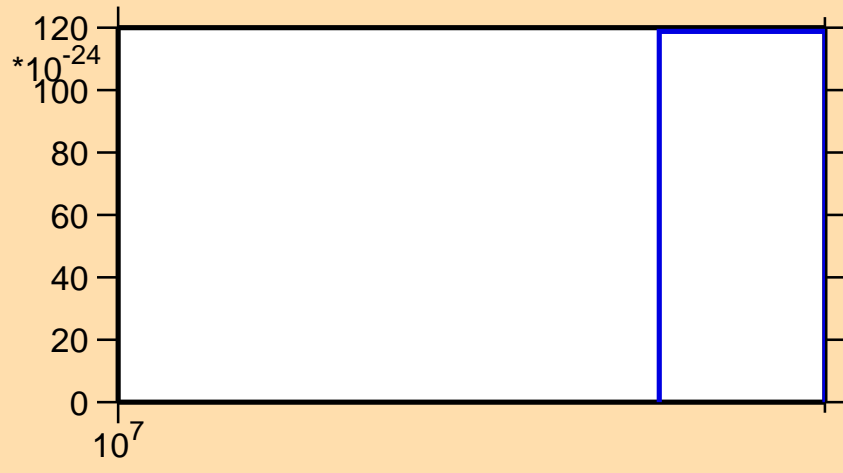
\sigma vs. E for ^{150}\text{Sm} (mt 11)
