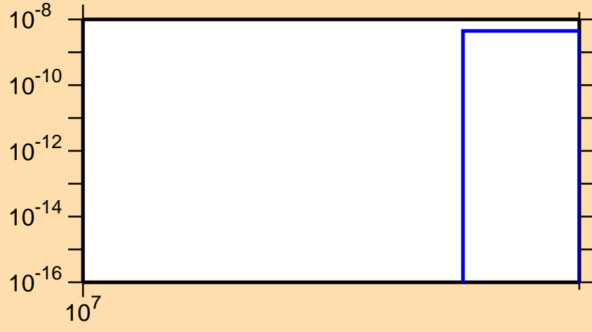
\sigma vs. E for ^{150}\text{Sm}(n,2np)
