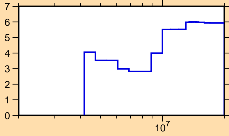
\Delta\sigma/\sigma vs. E for ^{150}\text{Sm}(n,\text{inel.})
