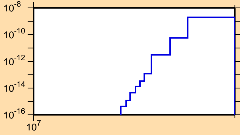
\sigma vs. E for ^{150}\text{Sm}(n,\text{He}3)
