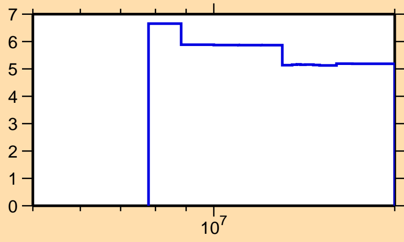
\Delta\sigma/\sigma vs. E for ^{150}\text{Sm}(n,2n)
