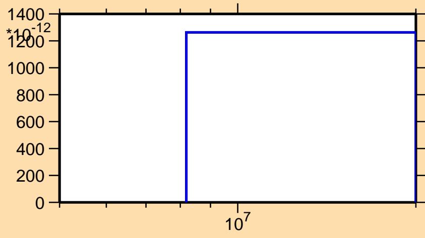
\sigma vs. E for ^{150}\text{Sm}(n,\text{nd})
