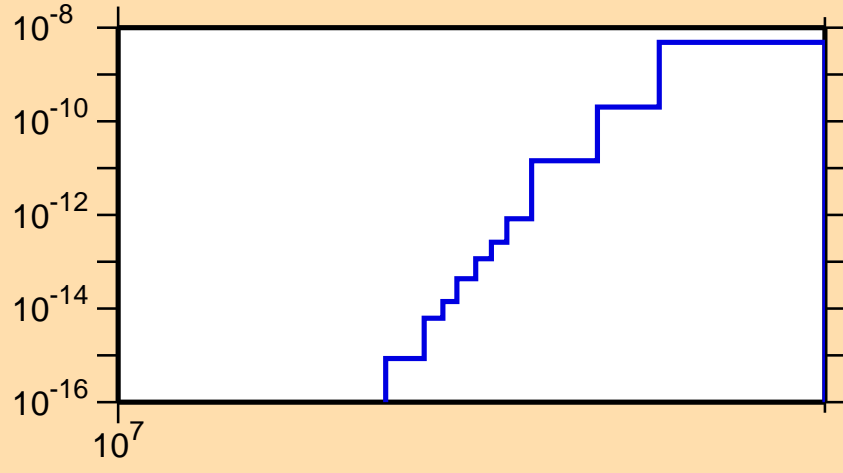
\sigma vs. E for ^{151}\text{Sm}(n,\text{He3})
