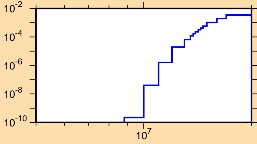
\sigma vs. E for ^{151}\text{Sm}(n,d)
