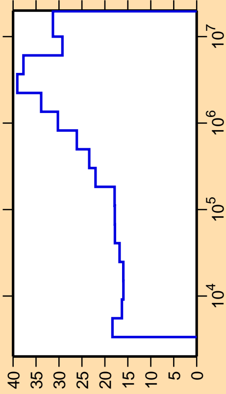
\Delta\sigma/\sigma vs. E for ^{151}\text{Sm}(n,\gamma)
