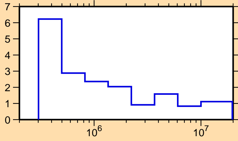
\Delta\sigma/\sigma vs. E for ^{151}\text{Sm}(n,\text{tot.})
