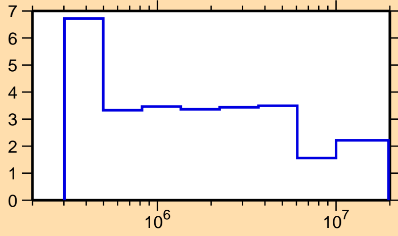
\Delta\sigma/\sigma vs. E for ^{151}\text{Sm}(n, el.)
