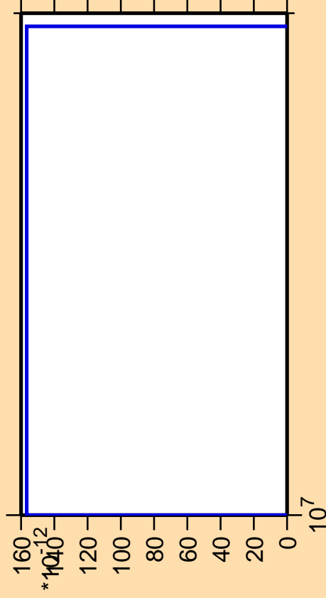
\Delta\sigma/\sigma vs. E for ^{151}\text{Sm} (mt 11)
