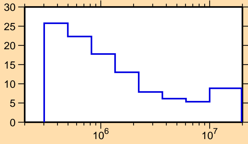
\Delta\sigma/\sigma vs. E for ^{151}\text{Sm}(n,n\text{cont.})
