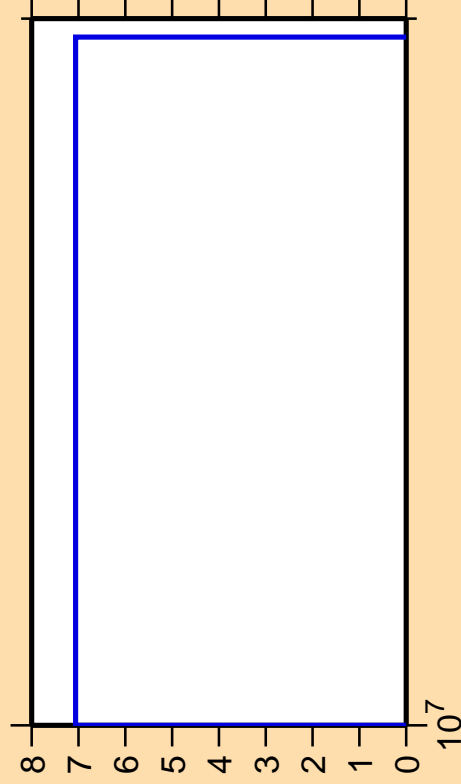
\Delta\sigma/\sigma vs. E for ^{151}\text{Sm}(n,3n)
