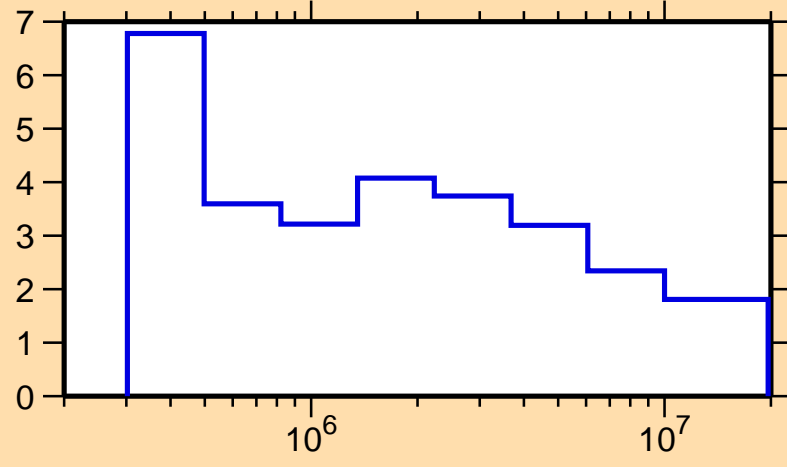
\Delta\sigma/\sigma vs. E for ^{151}\text{Sm}(n,\text{nonel.})
