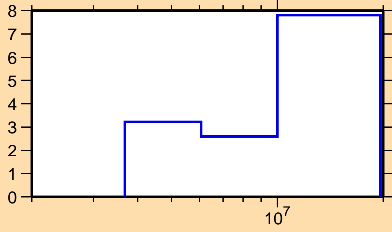
\Delta\sigma/\sigma vs. E for ^{151}\text{Sm}(n,\text{inel.})
