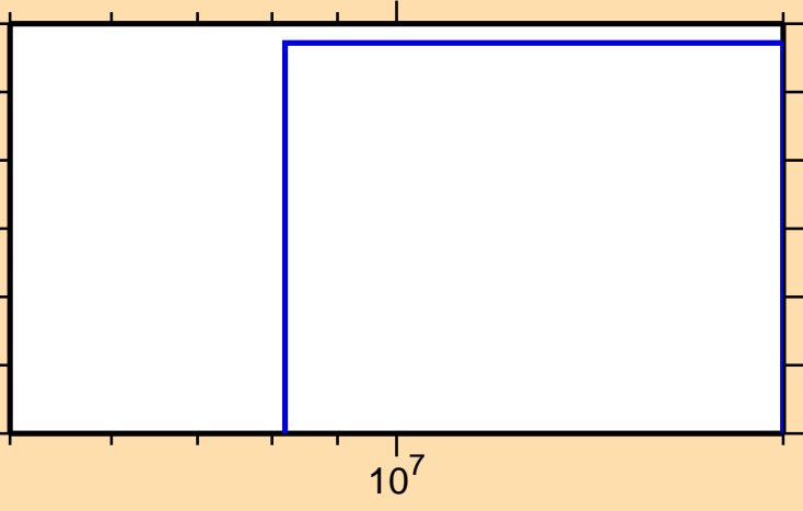
\sigma vs. E for ^{151}\text{Sm}(n,2np)
