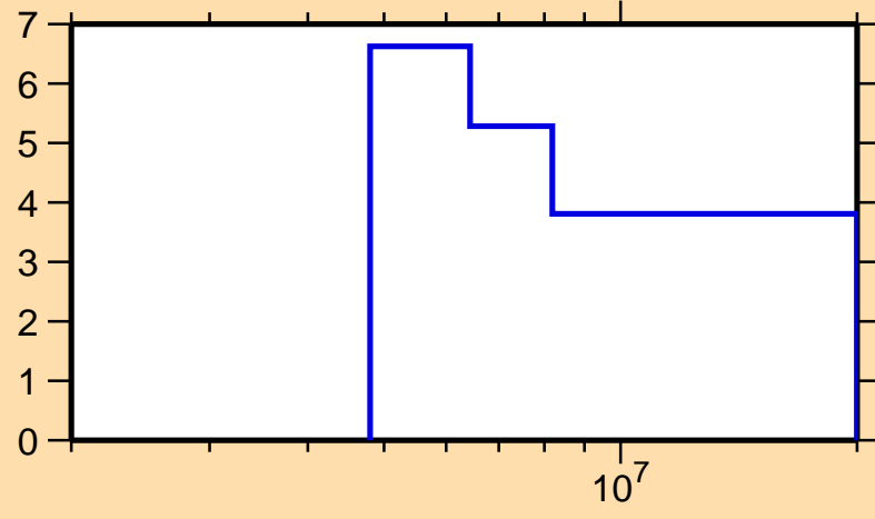
\Delta\sigma/\sigma vs. E for ^{151}\text{Sm}(n,2n)
