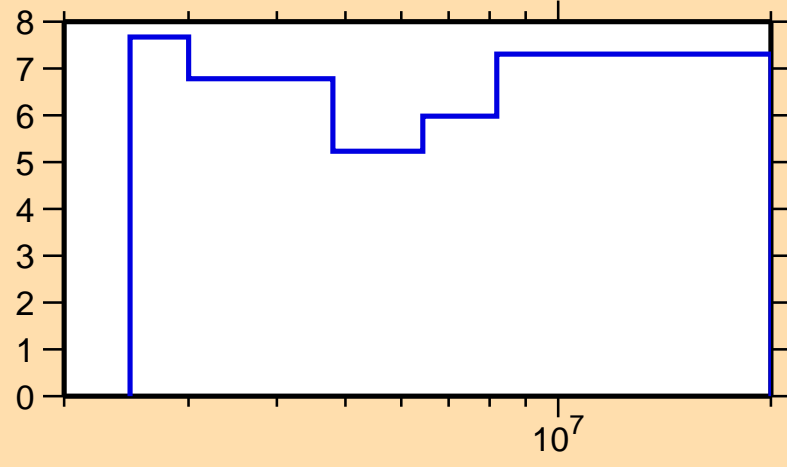
\Delta\sigma/\sigma vs. E for ^{151}\text{Sm}(n,n\text{cont.})
