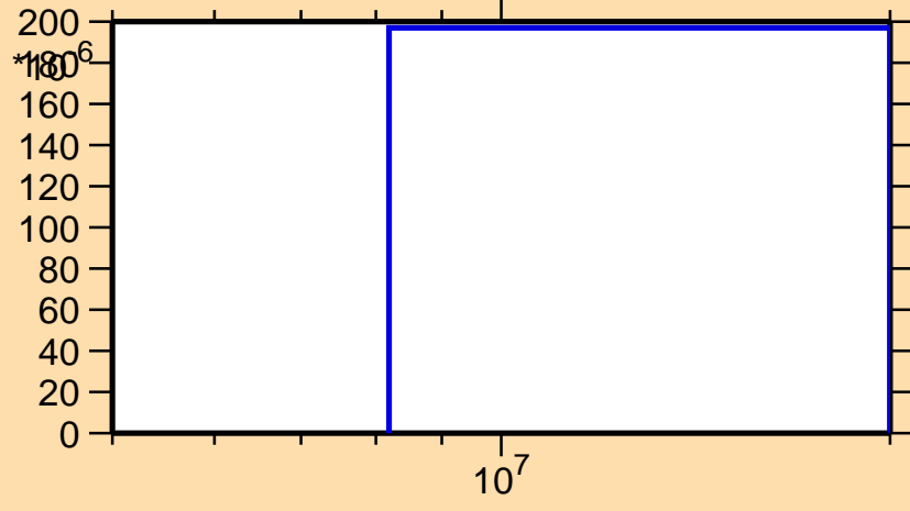
\sigma vs. E for ^{151}\text{Sm}(n,t)
