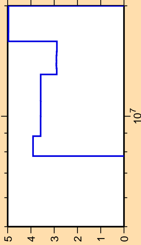
\Delta\sigma/\sigma vs. E for ^{152}\text{Sm}(n,2n)
