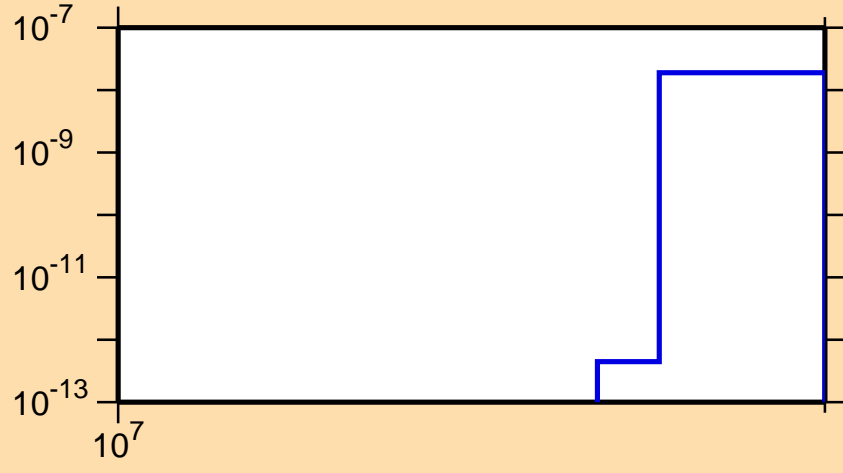
\sigma vs. E for ^{152}\text{Sm}(n,nt)
