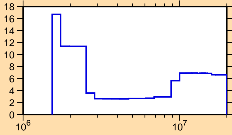
\Delta\sigma/\sigma vs. E for ^{152}\text{Sm}(n,ncont.)
