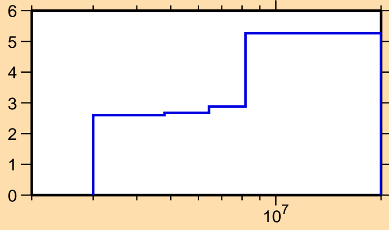
\Delta\sigma/\sigma vs. E for ^{152}\text{Sm}(n,n\text{cont.})
