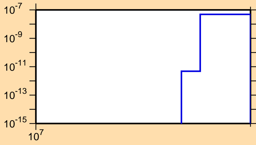
\sigma vs. E for ^{153}\text{Sm}(n,2np)
