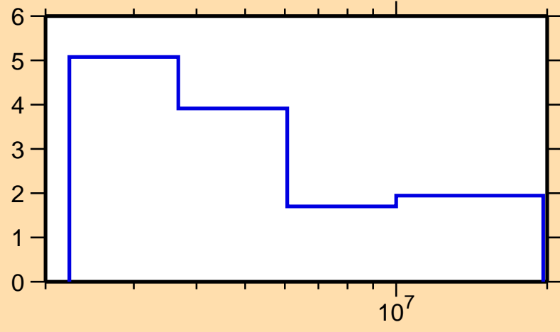
\Delta\sigma/\sigma vs. E for ^{153}\text{Sm}(n,el.)
