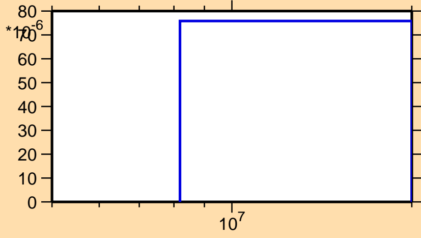
\sigma vs. E for ^{153}\text{Sm}(n,np)
