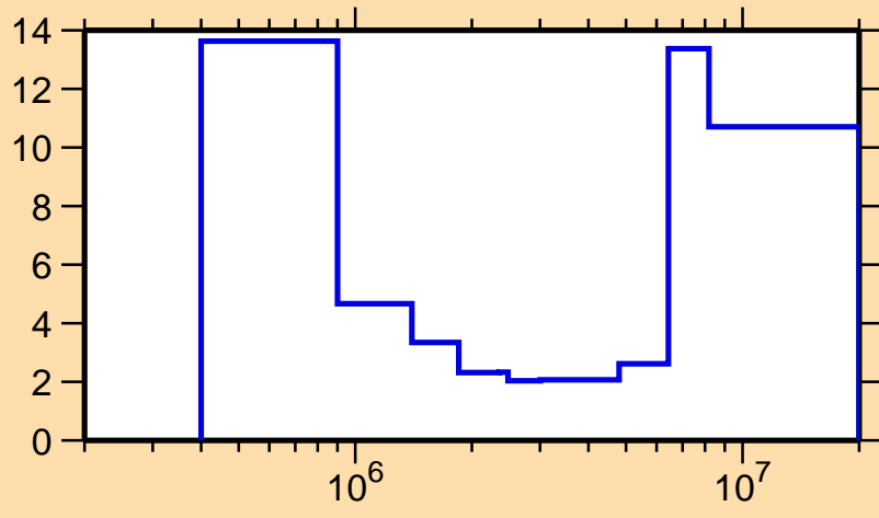
\Delta\sigma/\sigma vs. E for ^{153}\text{Sm}(n,\text{inel.})
