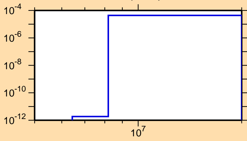
\sigma vs. E for ^{153}\text{Sm}(n,n\alpha)
