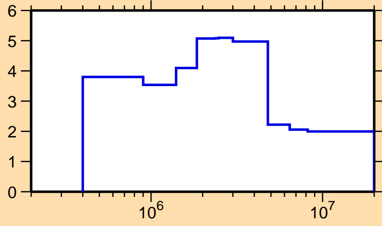
\Delta\sigma/\sigma vs. E for ^{153}\text{Sm}(n,\text{el.})
