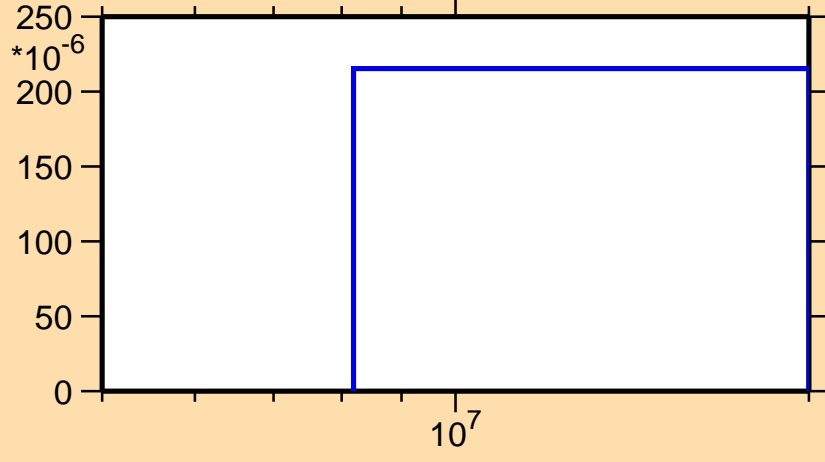
\sigma vs. E for ^{153}\text{Sm}(n,d)
