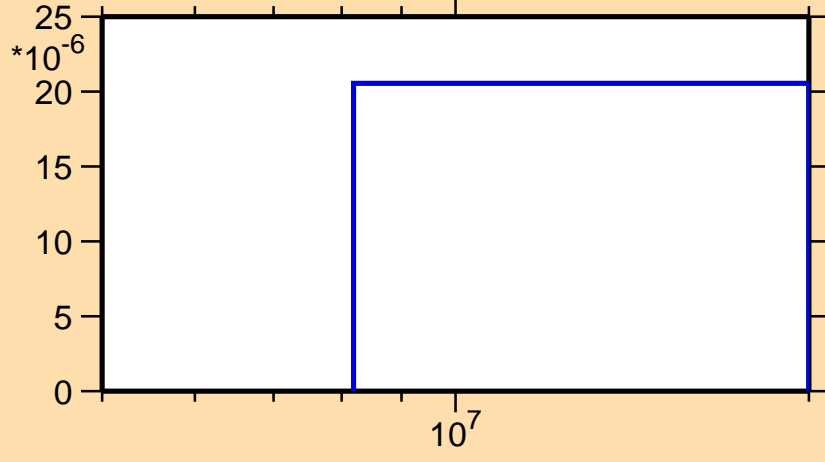
\sigma vs. E for ^{153}\text{Sm}(n,t)
