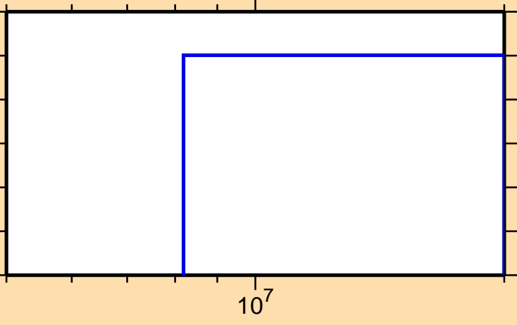
\sigma vs. E for ^{153}\text{Sm}(n,\text{nd})
