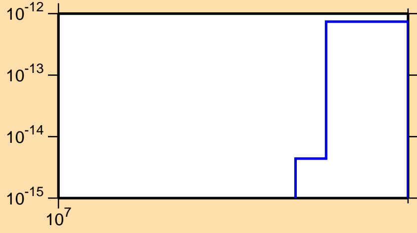
\sigma vs. E for ^{154}\text{Sm}(n,\text{He}3)
