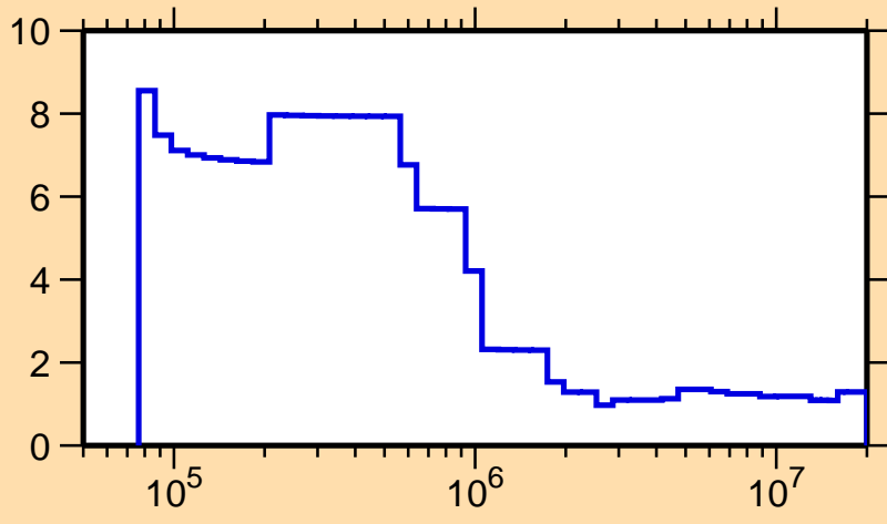
\Delta\sigma/\sigma vs. E for ^{154}\text{Sm}(n,\text{nonel.})
