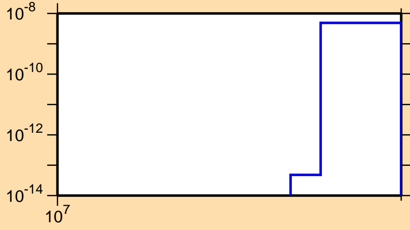
\sigma vs. E for ^{154}\text{Sm}(n,\text{nd})
