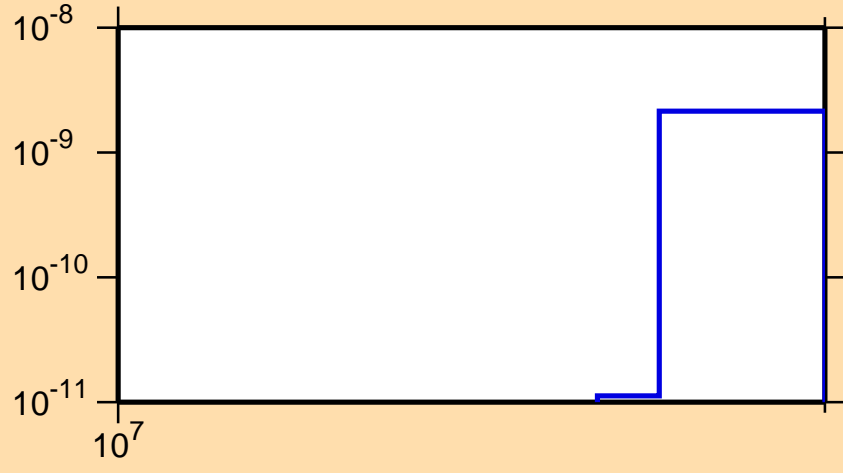
\sigma vs. E for ^{154}\text{Sm}(n,2n\alpha)
