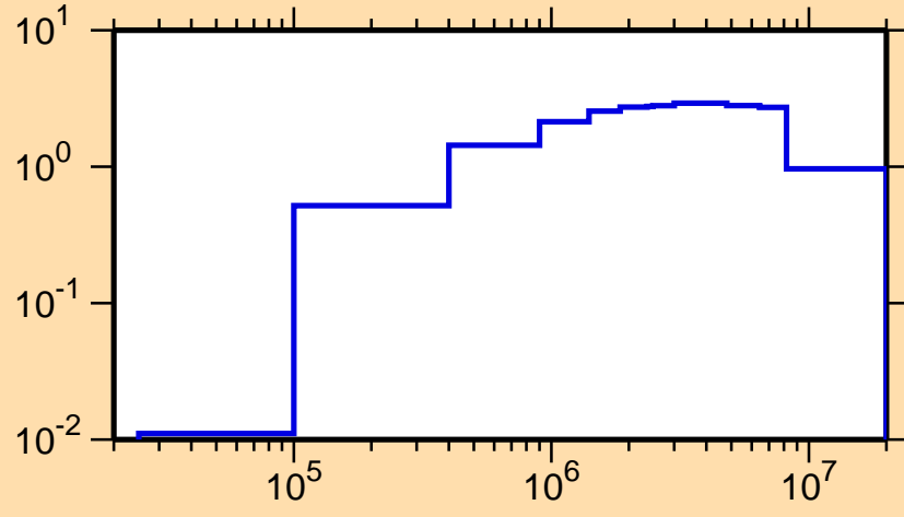
\sigma vs. E for ^{154}\text{Sm}(n,\text{inel.})
