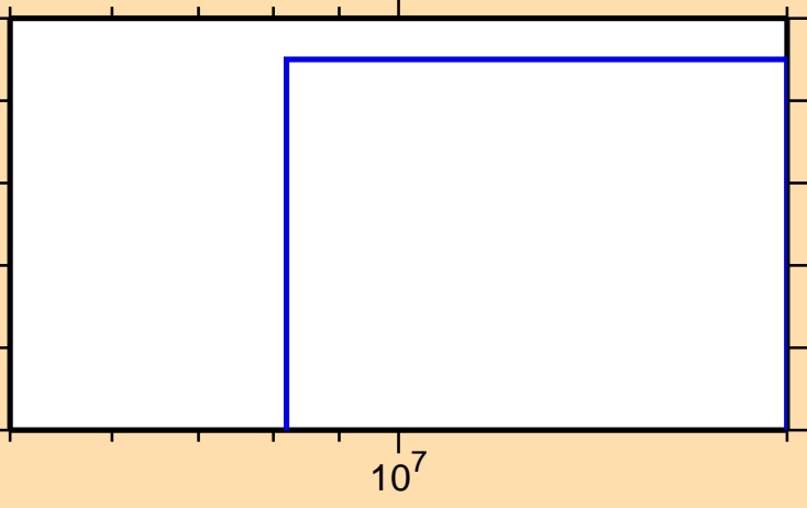
\sigma vs. E for ^{154}\text{Sm}(n,t)
