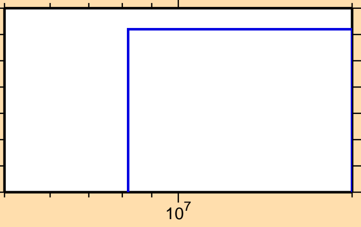
\sigma vs. E for ^{154}\text{Sm}(n,\text{He}3)
