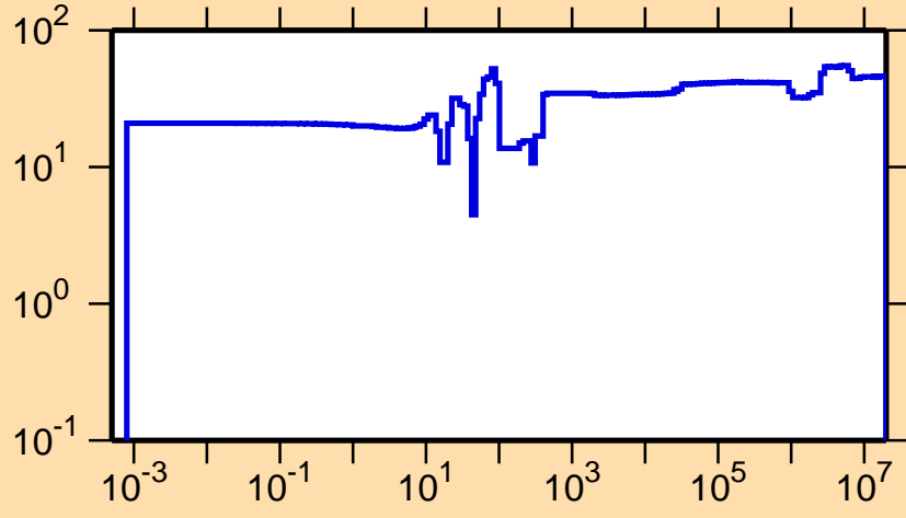
\Delta\sigma/\sigma vs. E for ^{155}\text{Sm}(n,\gamma)
