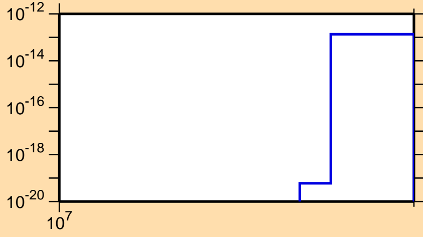
\sigma vs. E for ^{155}\text{Sm}(n,\text{He}3)
