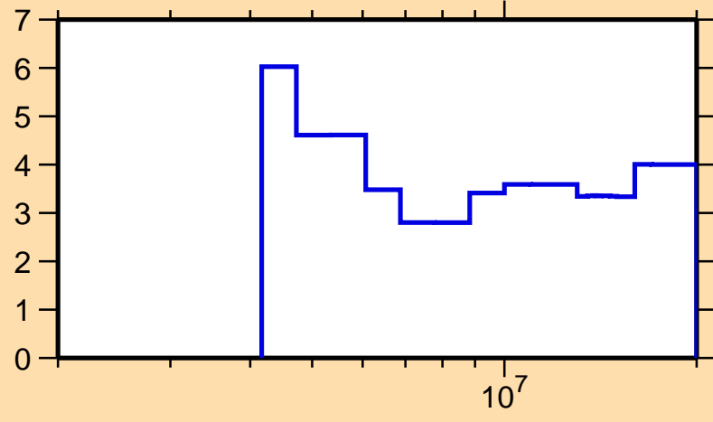
\Delta\sigma/\sigma vs. E for ^{155}\text{Sm}(n,el.)
