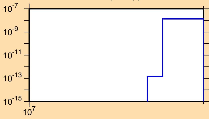
\sigma vs. E for ^{155}\text{Sm}(n,2np)
