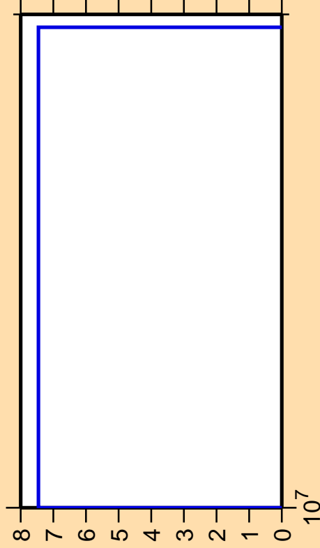
\Delta\sigma/\sigma vs. E for ^{155}\text{Sm}(n,3n)
