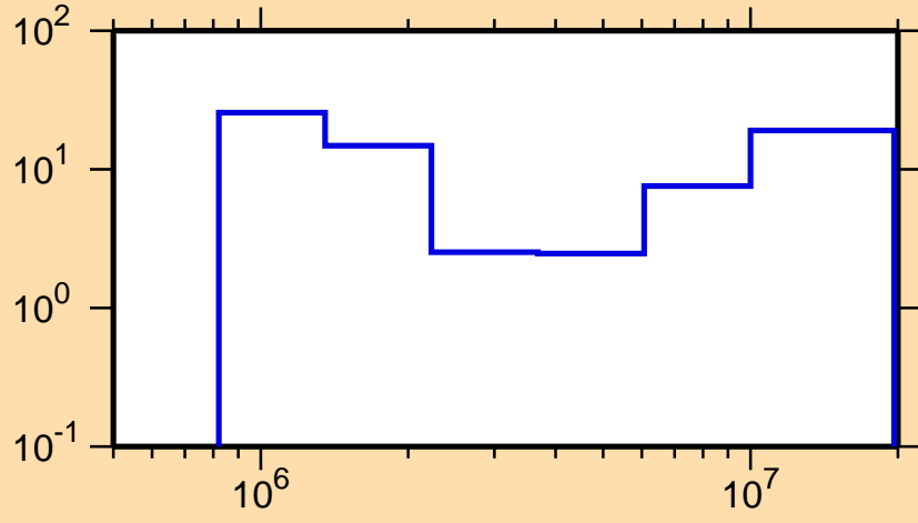
\Delta\sigma/\sigma vs. E for ^{155}\text{Sm}(n,n\text{cont.})
