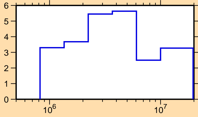
\Delta\sigma/\sigma vs. E for ^{155}\text{Sm}(n,\text{el.})
