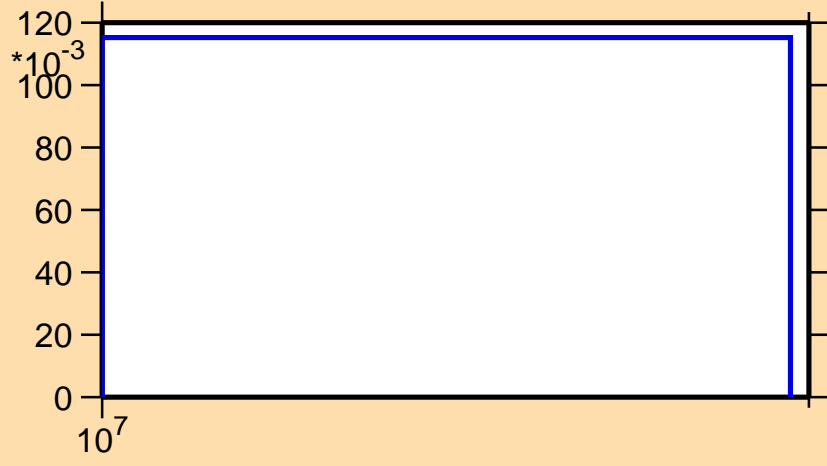
\sigma vs. E for ^{155}\text{Sm}(n,3n)
