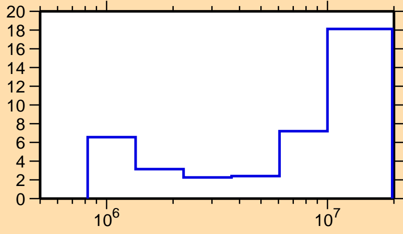
\Delta\sigma/\sigma vs. E for ^{155}\text{Sm}(n,\text{inel.})
