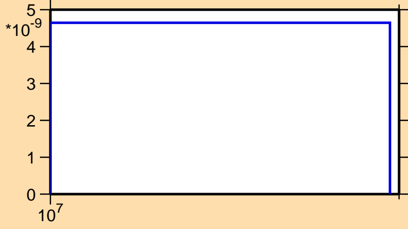
\sigma vs. E for ^{155}\text{Sm}(n,\text{nd})
