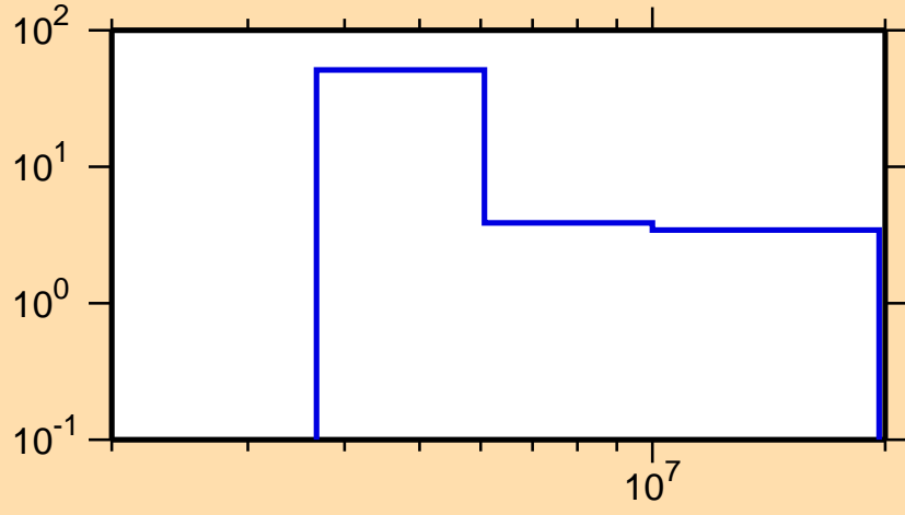
\Delta\sigma/\sigma vs. E for ^{155}\text{Sm}(n,2n)
