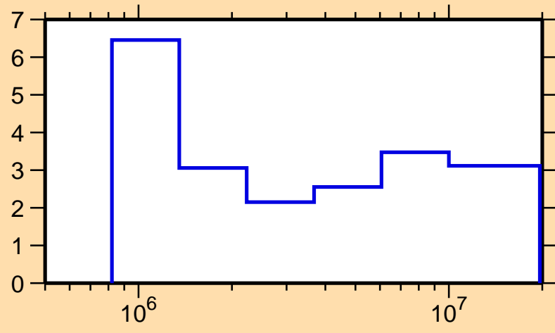
\Delta\sigma/\sigma vs. E for ^{155}\text{Sm}(n,\text{nonel.})
