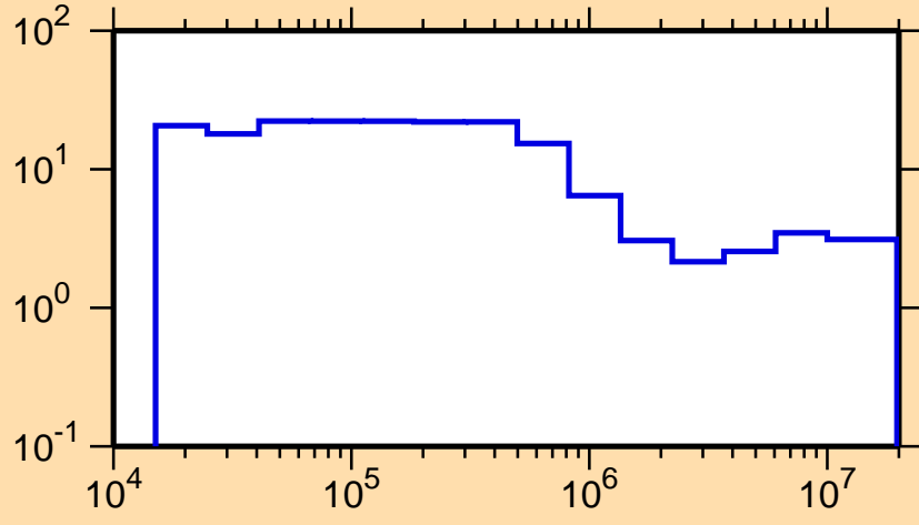
\Delta\sigma/\sigma vs. E for ^{155}\text{Sm}(n,\text{nonel.})
