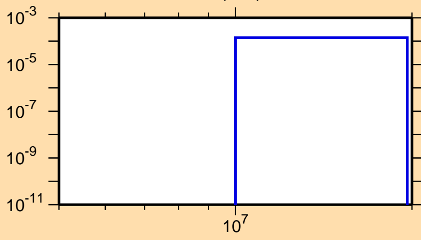
\sigma vs. E for ^{155}\text{Sm}(n,d)
