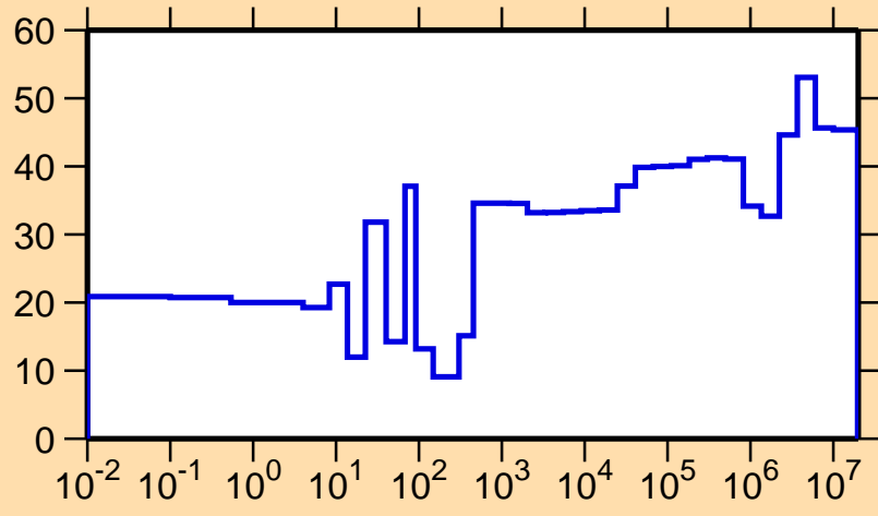
\Delta\sigma/\sigma vs. E for ^{155}\text{Sm}(n,\gamma)
