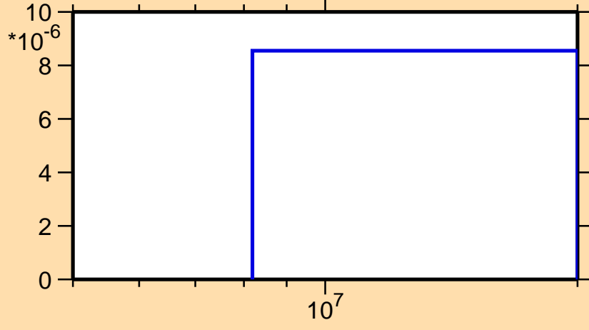
\sigma vs. E for ^{155}\text{Sm}(n,\alpha)
