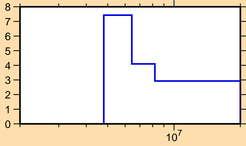
\Delta\sigma/\sigma vs. E for ^{155}\text{Sm}(n,2n)
