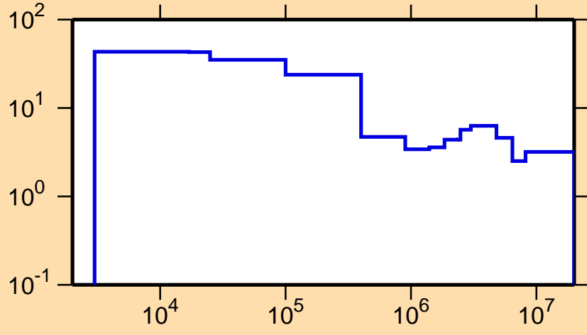
\Delta\sigma/\sigma vs. E for ^{155}\text{Sm}(n,el.)
