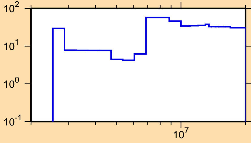
\Delta\sigma/\sigma vs. E for ^{156}\text{Sm}(n,n\text{cont.})
