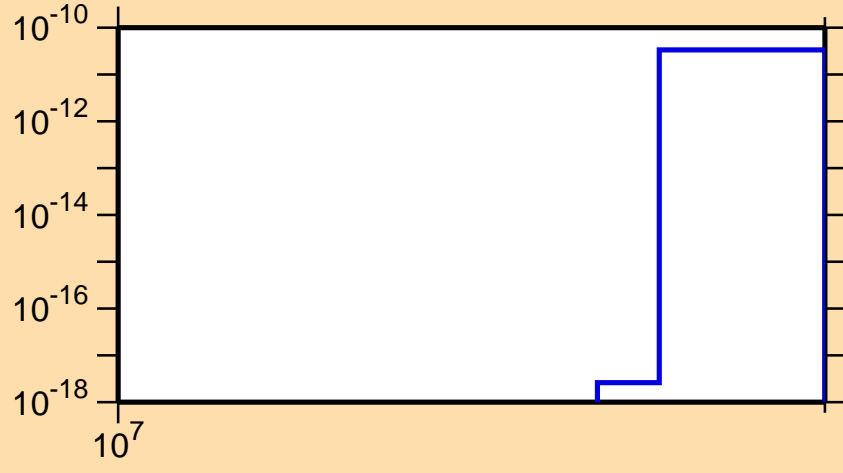
\sigma vs. E for ^{156}\text{Sm}(n,2np)
