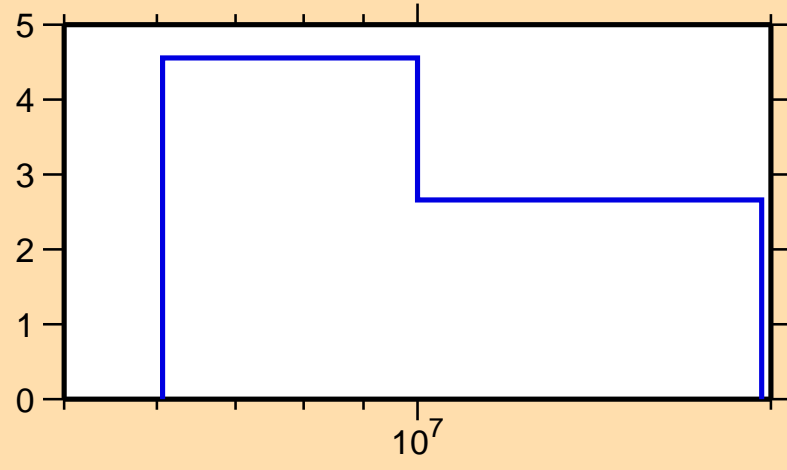
\Delta\sigma/\sigma vs. E for ^{156}\text{Sm}(n,\text{el.})
