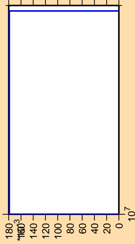
\Delta\sigma/\sigma vs. E for ^{156}\text{Sm}(n,2np)
